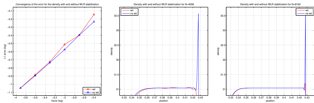
FIG. 10. Application of the WLR artificial viscosity method for our scheme in Test 7 : evolution of the error in L^1 -norm (left), zoom on the density for N = 4096 (center) and for N = 8192 (right).
