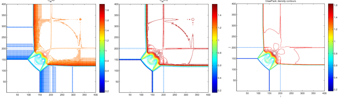
FIG. 11. Density contours (50 values) for 2D Riemann problem 3 computed with our scheme without WLR stabilization (left), with WLR stabilization (middle) and the reference solution from the Godunov method (right).
