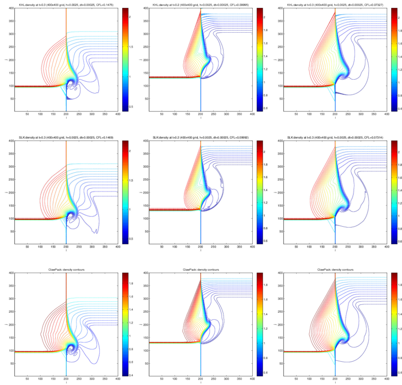
FIG. 9. Density contours (40) for 2D Riemann problems 17 to 19 with our scheme (first row), SLK scheme (second row) and Godunov method (third row).
