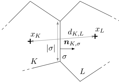
FIG. 1. Cell-centered finite-volume discretization.
