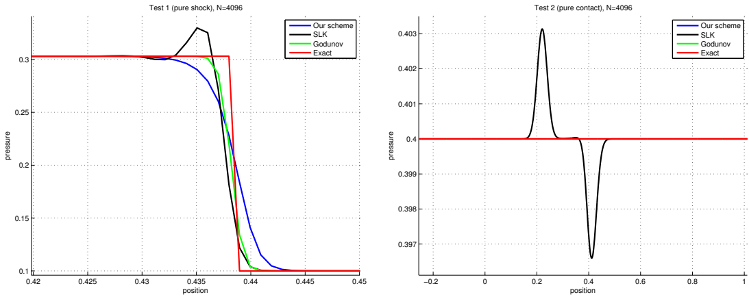
FIG. 3. Final state for Test 1 (left) and Test 2 (right) with our scheme (blue), the SLK scheme (black), the Godunov method (green) and the exact solution (red). The mesh size is h = 8/4096 .
