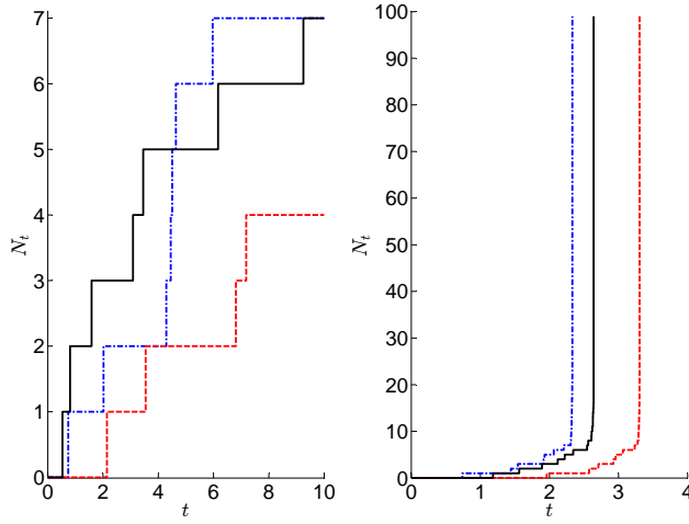
Fig. 2 A few trajectories of (N_t)_{t \geq 0} for \Lambda(t) = t^{1.25} with h(n) = 0.75^n (left) and h(n) = 1.5^n (right)
