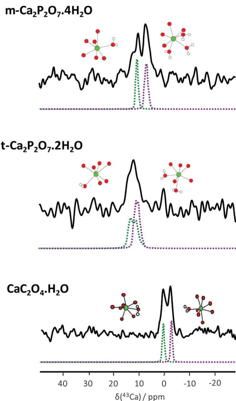
Fig. 2 Natural abundance ^{43}\text{Ca} MAS NMR spectra of m\text{-Ca}_2\text{P}_2\text{O}_7\cdot 4\text{H}_2\text{O} (m-CPPT \beta , 2.5 hours), t\text{-Ca}_2\text{P}_2\text{O}_7\cdot 2\text{H}_2\text{O} (t-CPPD, 3 hours) and \text{CaC}_2\text{O}_4\cdot \text{H}_2\text{O} (COM, 3 hours), recorded at 35.2 T. The dashed lines show the simulation of the contributions of the two inequivalent Ca-sites in each structure, using the experimental ^{43}\text{Ca} NMR parameters determined previously (which are recalled in ESI† in Table S2). 2,3
