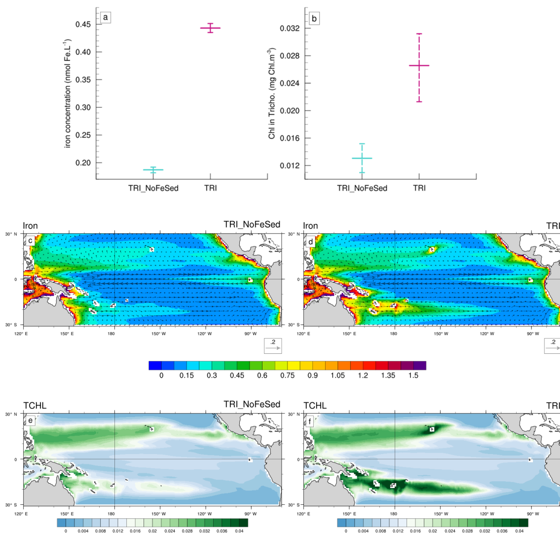
Figure 9. (a, b) Minimum, mean and maximum in the South box (Fig. 1c) of (a) the iron concentrations (in nmol Fe L -1 ), and (b) of the chlorophyll concentrations of Trichodesmium (in mg Chl m -3 ). (c, d, e, f) Annual mean iron concentrations (shading; in nmol Fe L -1 ) and current velocities (vectors; in m s -1 ) for (c) the TRI_NoFeSed simulation and (d) the TRI simulation. Annual mean chlorophyll concentrations of Trichodesmium (mg Chl m -3 ) for (e) the TRI_NoFeSed simulation and (f) the TRI simulation. The concentrations have been averaged over the top 100 m of the ocean. The current velocities are identical on the panels (a) and (b).
