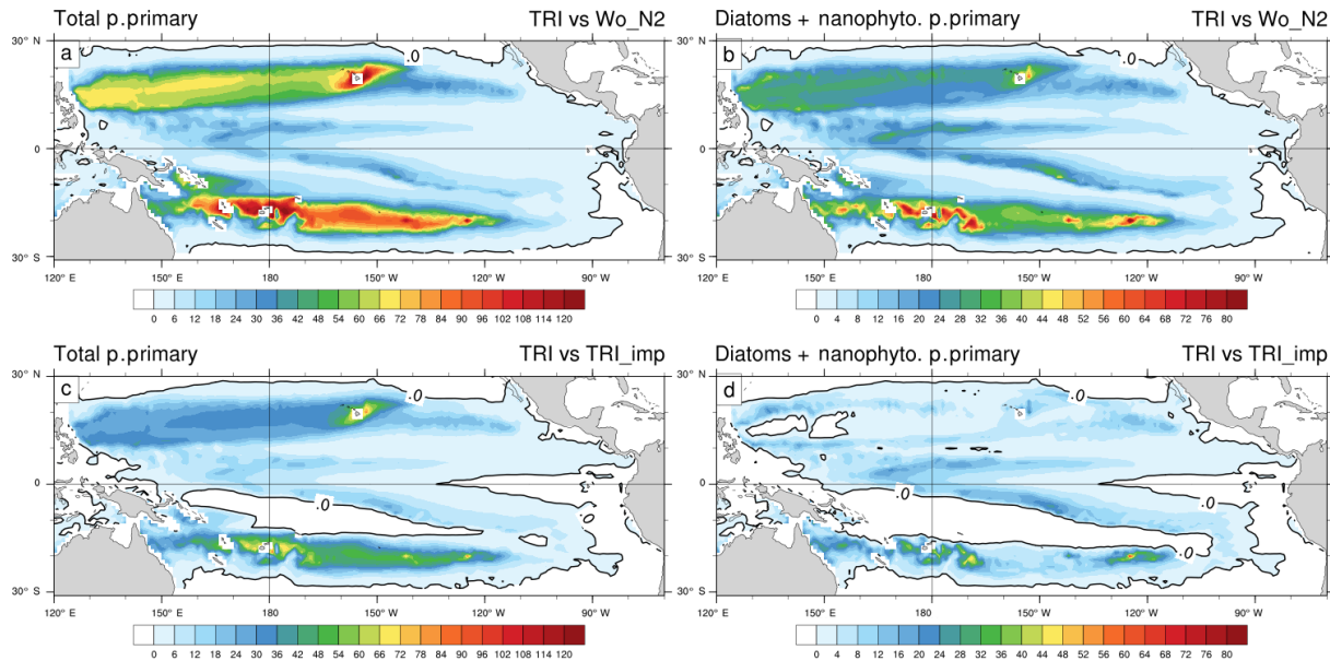
Figure 10. Percentage increase in primary production between the TRI simulation and the Wo_N2 simulation ( a , b ) and the TRI_imp simulation ( c , d ); panels ( a ) and ( c ) show total primary production including the contribution of Trichodesmium whereas in panels ( b ) and ( d ), primary production only includes the contribution of diatoms and nanophytoplankton.
