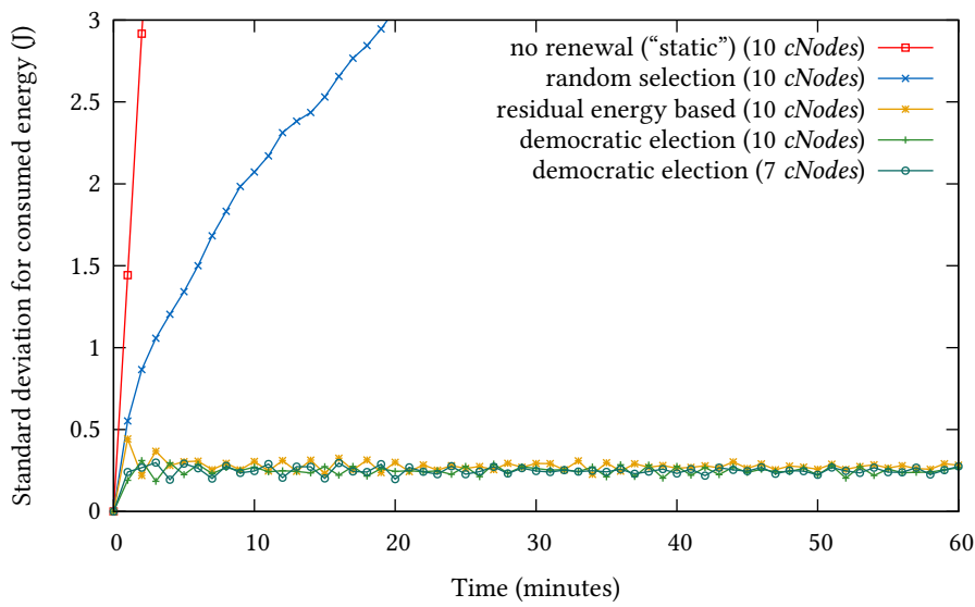
Figure 8. Standard deviation for the energy consumed by sensors in function of elapsed time (initial energy amount: \infty )
