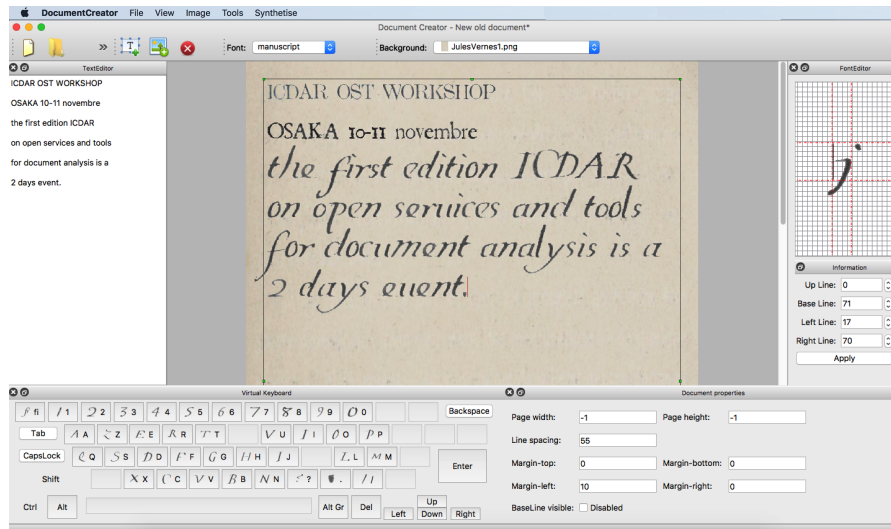
Fig. 4. GUI of DocCreator (desktop version). The central windows allows to input text to compose interactively synthetic document images using aivable fonts and backgrounds. On the left, the original text is present. On the right, one can edit the properties of a character of the font. On the bottom, the mapping of the font onto the physical keyboard is presented via a virtual keyboard. One can also edit global properties of the document. Defect models are available in the top menu. Batch generation is available through “the factory” icon on the toolbar. An online version is also available at http://doc-creator.labri.fr/ . The different features available on online/desktop latests versions are listed on the web site.
