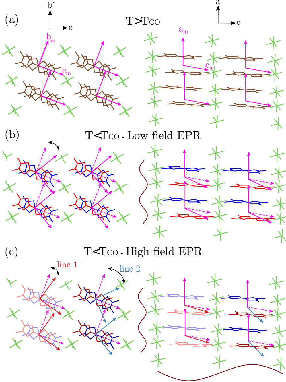
Figure 5: (color online). Schematic representation of the structural and magnetic properties of (\text{TMTTF})_2\text{X} . The left column represents 4 unit cells in the plane perpendicular to the chain axis a while the right side is 4 unit cells in the plane ac . (a) At T > T_{CO} , the charge density is equally distributed between the TMTTF molecules (brown). The principal axis of the g -tensor (pink) are oriented along the TMTTF molecular axes. All the unit cells are magnetically equivalent. (b) At T < T_{CO} the charge density of the two TMTTF molecules is no more balanced and the g -tensor axes rotate about the a axis 20 . (c) The high-field/high-frequency EPR experiments reveal that this rotation is not uniform due to modulation of the charge ordering. The charge unbalance is stronger in one stack (dark blue and red) than in the second (light blue and red) leading to two different rotations of the g -tensor axes and thus to two EPR lines.
