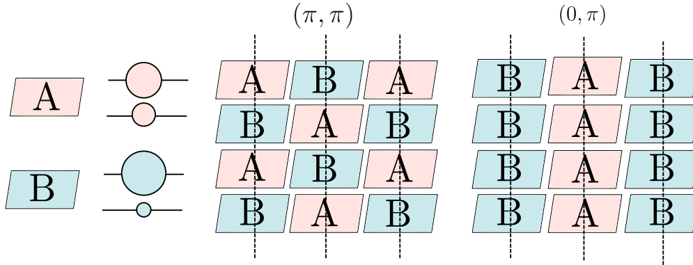
Figure 3: (color online). Schematic representation of CO superlattice inspired from the original work of Riera and Poilblanc 4 . A and B are unit cells of (\text{TMTTF})_2X in the CO configuration (ie : with charge density displacement) but B has a stronger charge displacement than A. The vertical dashed lines represent the chain axis. The (\pi, \pi) configuration alternates A and B in both directions whereas (0, \pi) has a uniform A or B inside the chain but alternates between the chains.
