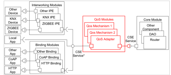
Fig. 6. Internal structure of an OM2M node integrating QoS-oriented modules
