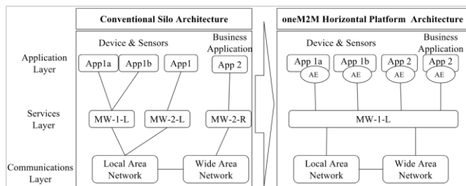
Fig. 3. oneM2M's horizontal architecture (providing a unifying framework for silo applications)
