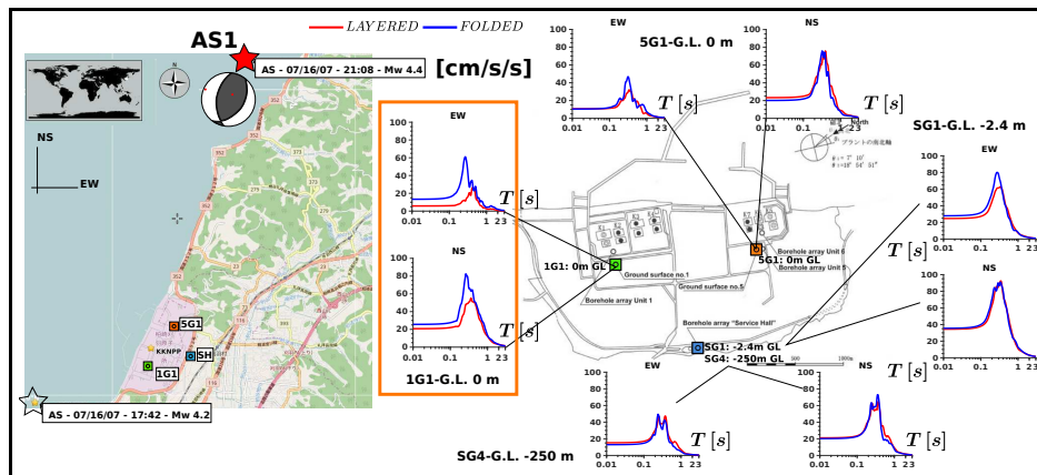
Figure 7: AS1: response spectra ( S_a , in cm/s^2 ) at different locations around the KKNPP site. LAYERED (red) and FOLDED geological models were compared.
