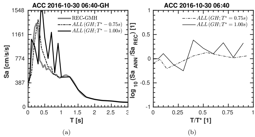
Figure 10: (a) Recorded (thick gray line) and estimated Sa spectra (geometric mean of the horizontal components), for T^*=0.75\text{ s} (dashed black line) and T^*=1\text{ s} (solid black line). (b) ANN performance for different training corner periods T^* (0.75 and 1 s respectively), expressed in terms of estimated/target Sa . The data refer to stations ACC, which recorded the CIT2016
