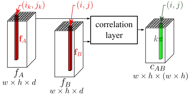
Fig. 3. Correlation map computation with CNN features. The correlation map c_{AB} contains all pairwise similarities between individual features \mathbf{f}_A \in f_A and \mathbf{f}_B \in f_B . At a particular spatial location (i, j) the correlation map output c_{AB} contains all the similarities between \mathbf{f}_B(i, j) and all \mathbf{f}_A \in f_A .
