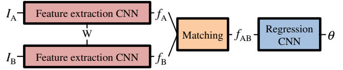
Fig. 2. Diagram of the proposed architecture. Images I_A and I_B are passed through feature extraction networks which have tied parameters W , followed by a matching network which matches the descriptors. The output of the matching network is passed through a regression network which outputs the parameters of the geometric transformation.
