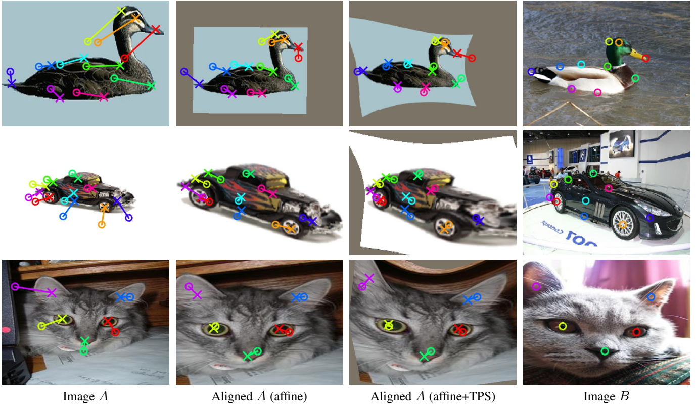
Fig. 9. Qualitative results on the PF dataset. Each row shows one test example from the Proposal Flow dataset. Ground truth matching keypoints, only used for alignment evaluation, are depicted as crosses and circles for images A and B , respectively. Keypoints of same color are supposed to match each other after image A is aligned to image B . To illustrate the matching error, we also overlay keypoints of B onto different alignments of A so that lines that connect matching keypoints indicate the keypoint position error vector. Our method manages to roughly align the images with an affine transformation (column 2), and then perform finer alignment using thin-plate spline (TPS, column 3). The top two examples are from the PF-WILLOW dataset while the bottom one is from PF-PASCAL.
