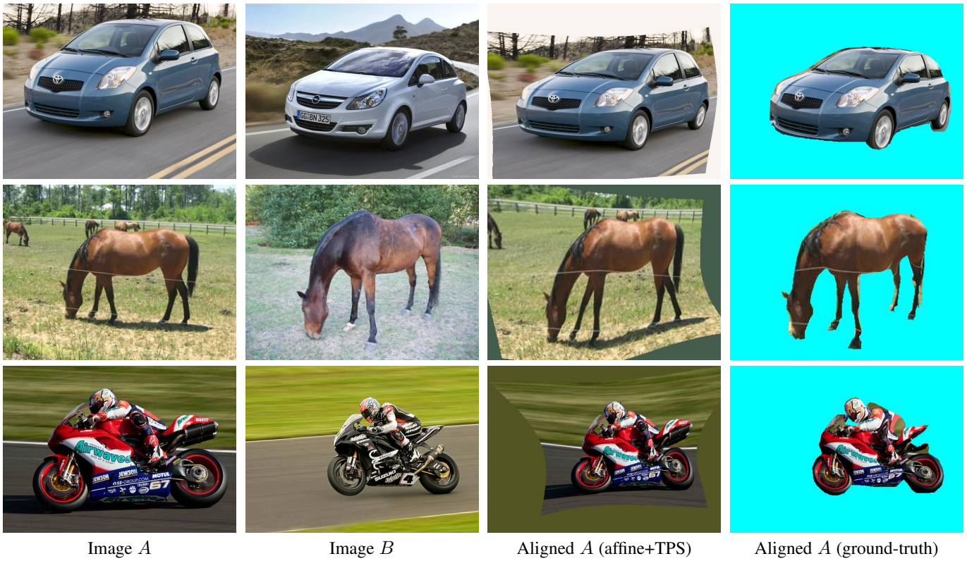
Fig. 10. Qualitative results on the TSS dataset. Each row shows one test example from the TSS dataset. The last column shows the ground-truth alignment used for evaluation. Example 1 is from TSS-FG3DCar, examples 2-3 are from TSS-JODS, and 4-7 from TSS-PASCAL.
