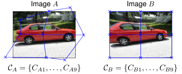
Fig. 5. Thin-plate spline control points. Illustration of the 3 \times 3 TPS grid of control points used in the thin-plate spline transformation model.
