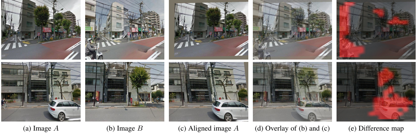
Fig. 14. Qualitative results on the Tokyo Time Machine dataset. Each row shows a pair of images from the Tokyo Time Machine dataset, and our alignment along with a “difference map”, highlighting absolute differences between aligned images in the descriptor space. Our method successfully aligns image A to image B despite of viewpoint and scene changes (highlighted in the difference map).
