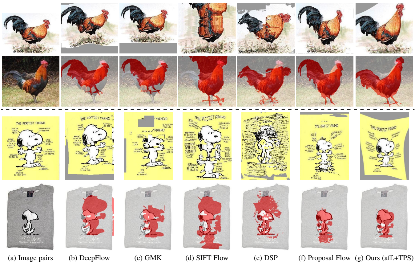
Fig. 11. Qualitative results on the Caltech-101 dataset. Each block of two rows corresponds to one example, where column (a) shows the original images – image A in the first row and image B in the second row. The remaining columns of the first row show image A aligned to image B using various methods. The second row shows image B overlaid with the segmentation map transferred from image A.
