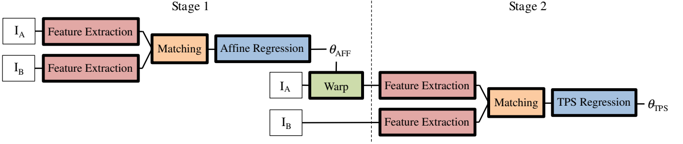
Fig. 6. Estimating progressively more complex geometric transformations. Images A and B are passed through a network which estimates an affine transformation with parameters \theta_{\text{AFF}} (see Fig. 2). Image A is then warped using this transformation to roughly align it with B , and passed along with B through a second network which estimates a thin-plate spline (TPS) transformation that refines the alignment.
