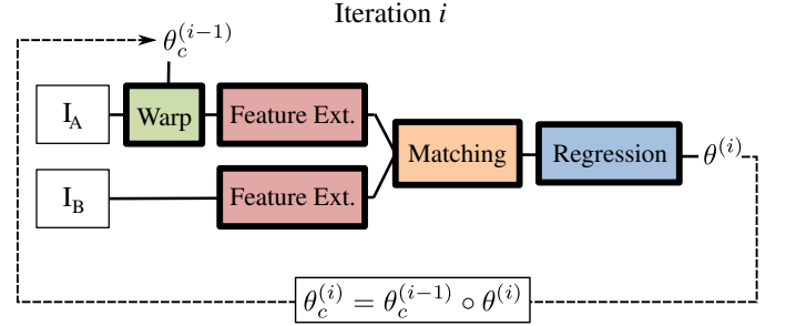
Fig. 7. Iterative transformation refinement. In iteration i , image A is warped using the cumulative transformation estimate \theta_c^{(i-1)} obtained from the previous iteration ( \theta_c^{(0)} is initialized to identity). A fine alignment, \theta^{(i)} , between image B and the warped image A is estimated and chained onto \theta_c^{(i-1)} to form the refined cumulative transformation estimate \theta_c^{(i)} .
