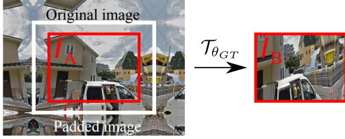
Fig. 8. Synthetic image generation. Symmetric padding is added to the original image to enlarge the sampling region, its central crop is used as image A , and image B is created by performing a randomly sampled transformation \mathcal{T}_{\theta_{GT}} .
