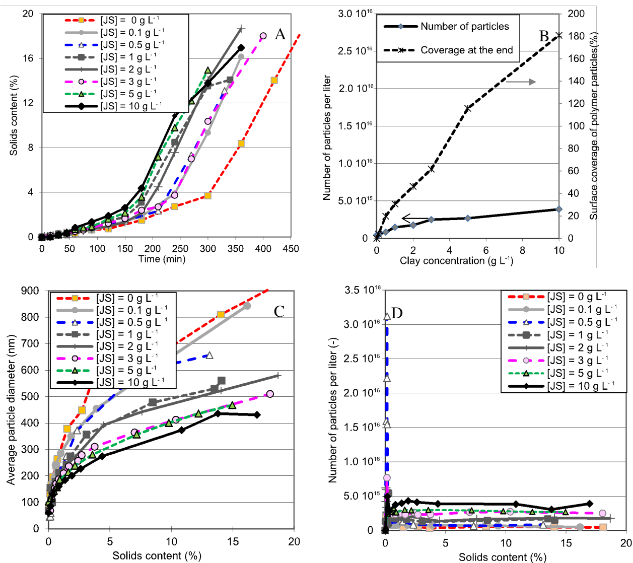
Figure 5. Pickering ab initio semi-continuous emulsion polymerization of styrene stabilized by different amounts of Laponite JS.
