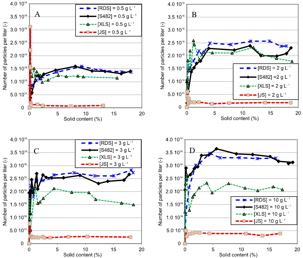
Figure 6. Comparison of the different clay grades in Pickering ab initio semi-continuous emulsion polymerization of styrene for different amounts of Laponite: (A) 0.5 g L -1 , (B) 2.0 g L -1 , (C) 3.0 g L -1 , and (D) 10.0 g L -1 .
