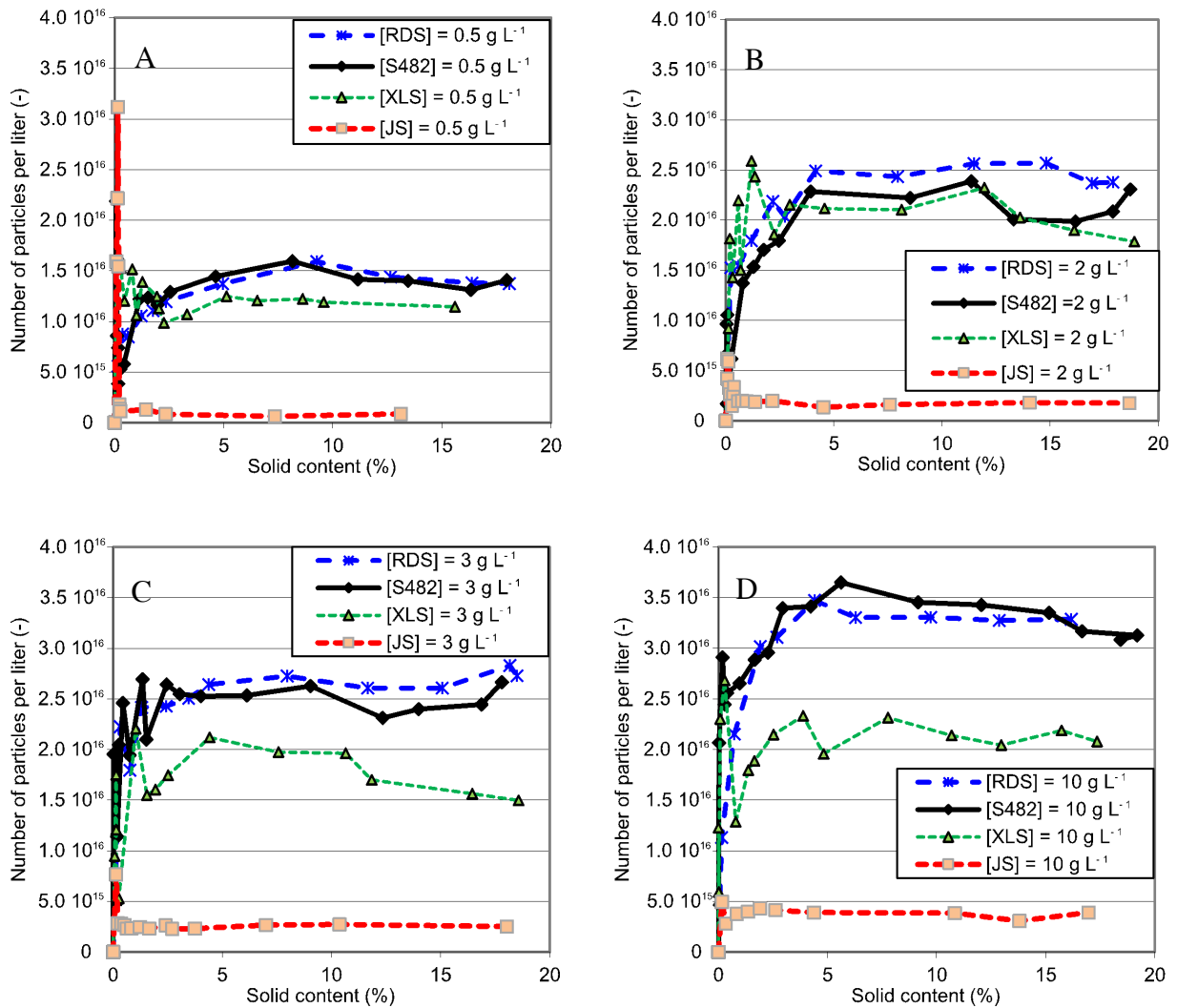
Figure 6. Comparison of the different clay grades in Pickering ab initio semi-continuous emulsion polymerization of styrene for different amounts of Laponite: (A) 0.5 \text{ g L}^{-1} , (B) 2.0 \text{ g L}^{-1} , (C) 3.0 \text{ g L}^{-1} , and (D) 10.0 \text{ g L}^{-1} .
