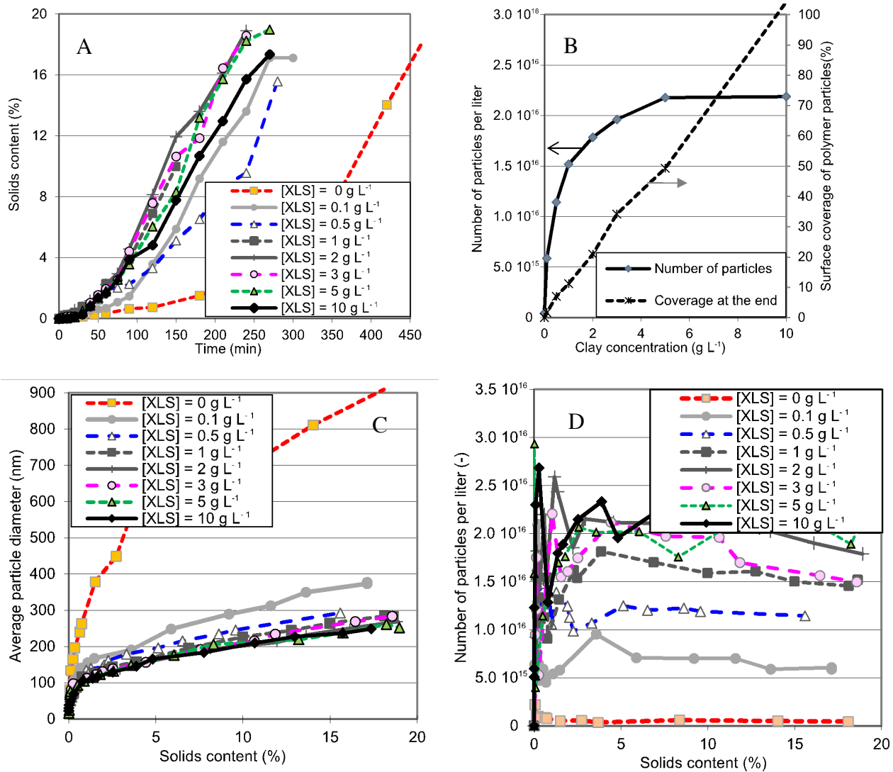
Figure 4. Pickering ab initio semi-continuous emulsion polymerization of styrene stabilized by different amounts of Laponite XLS.
