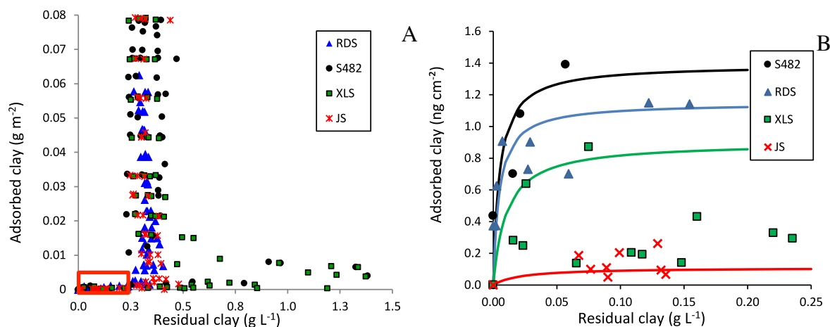
Figure 1. A: Adsorption isotherm of Laponite clay platelets on preformed polystyrene latex particles (with 5 wt% solids content and mean diameter 300 nm) measured using ICP-AES based on Si analysis and B: Zoom of the selected zone in Figure A with Langmuir fits (continuous line).
