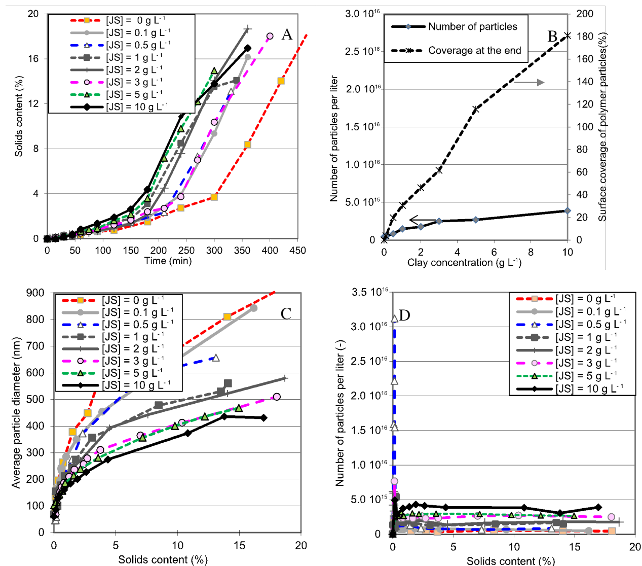
Figure 5. Pickering ab initio semi-continuous emulsion polymerization of styrene stabilized by different amounts of Laponite JS.
