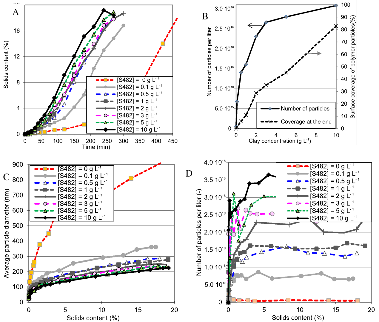
Figure 3. Pickering ab initio semi-continuous emulsion polymerization of styrene stabilized by different amounts of Laponite S482.
