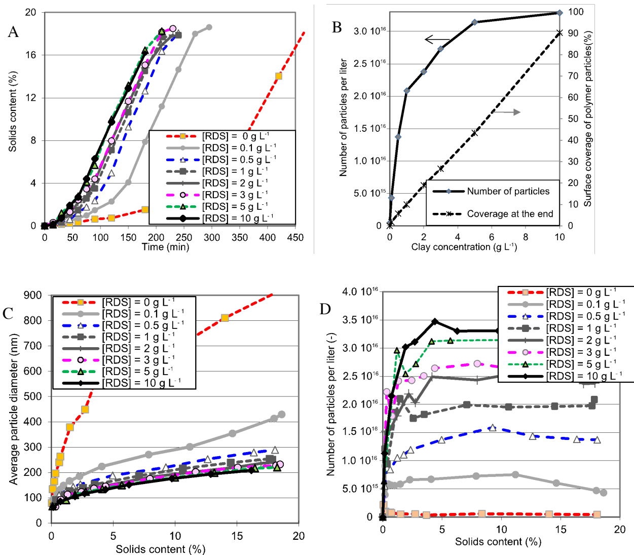
Figure 2. Pickering ab initio semi-continuous emulsion polymerization of styrene stabilized by different amounts of Laponite RDS. Reprinted with permission from Langmuir , 2016, 32, 112–124, copyright 2016 American Chemical Society.
