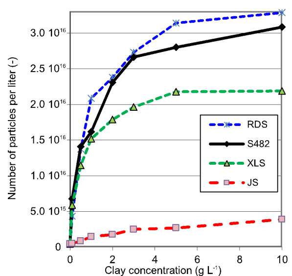
Figure 7. Comparative summary of the behaviors of the four Laponite clays in emulsion polymerization.
