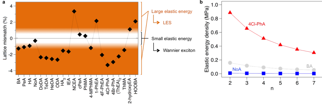
Figure 5: Design of LHPs for photovoltaics and optoelectronics. (a) Lattice mismatch between various monolayered A'_{2}PbI_{4} perovskites ( n=1 ) and MAPbI_{3} ( I4cm ; n=\infty ). All data are taken from X-ray structures resolved at room-temperature. Names for organic compounds and corresponding references are given Table S4 (SI). (b) Computed elastic energy density for heterostructures built with MAPbI_{3} and (BA)_{2}PbI_{4} (grey line), (C_{9}H_{19}NH_{3})_{2}PbI_{4} (NoA, blue line), and (4Cl-C_{6}H_{4}NH_{3})_{2}PbI_{4} (4Cl-PhA, red line).
