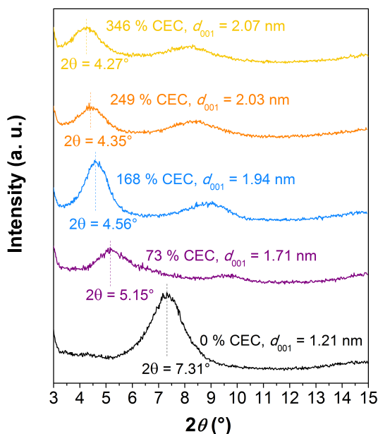
Figure 3. XRD patterns of MMT/P(DMAEMA 26 - co -BA 20 )-CTPPA complexes for increasing amounts of adsorbed macroRAFT agent expressed as percentage of the cation exchange capacity (CEC) of MMT (MMT = 5.0 g L -1 ).
