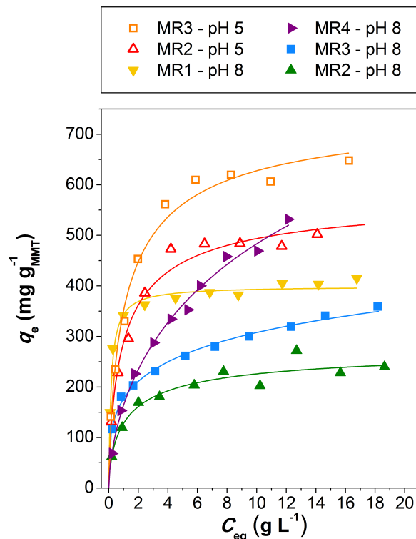
Figure 1. Experimental equilibrium adsorption isotherms of anionic and non-ionic macroRAFT agents onto MMT at pH 8 and pH 5 ( \text{MMT} = 5.0 \text{ g L}^{-1} ) at ambient temperature. MR3 - P( \text{AA}_9\text{-co-PEGA}_9\text{-co-BA}_9 )-CTPPA ( \square , pH 5 and \blacksquare , pH 8), MR2 - P( \text{AA}_4\text{-co-PEGA}_4\text{-co-BA}_4 )-CTPPA ( \triangle , pH 5 and \blacktriangle , pH 8), MR1 - P( \text{PEGA}_4\text{-co-BA}_3 )-CTPPA ( \nabla , pH 8) and MR4 - P( \text{AA}_{41}\text{-b-P(PEGA}_6\text{-co-BA}_4 )-CTPPA ( \blacktriangleright , pH 8) (see Table 3 for details). The lines are the best fits to Sips model.
