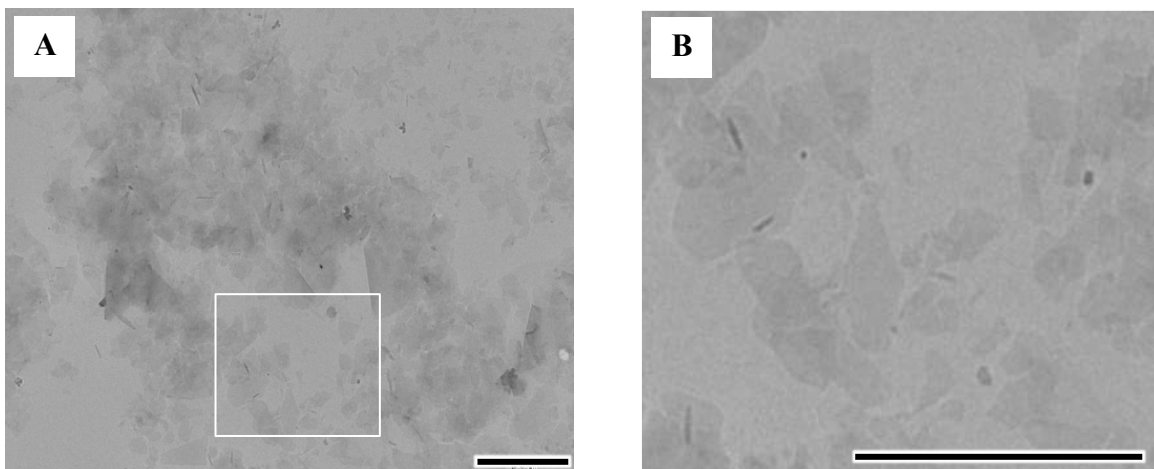
Figure 5. (A) TEM images of MMT/P(DMAEMA 17-co -PEGA 7-co -BA 19 )-CTPPA ([MMT] = 5.0 g L -1 ; [macroRAFT agent] = 6.5 g L -1 ). (B) Zoom of insert in Figure A. Scale bars: 1 μm.
