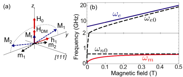
FIG. 1. (color online) (a) Magnetic structure of antiferromagnetic \text{MnCO}_3 in the (111) plane ( y - z plane). Electron magnetic sublattices with magnetizations M_1 and M_2 , respectively, are slightly canted due to the Dzyaloshinskii-Moriya interaction represented by the effective magnetic field H_{DM} . As a result, the non-zero net magnetization M_f causes weak ferromagnetism of \text{MnCO}_3 . Nuclear magnetic sublattices with magnetizations m_1 and m_2 , respectively, are coupled to the electron sublattices through the hyperfine interaction fields \mathbf{H}_n = -A\mathbf{M}_i ( i = 1, 2 ). H_0 is the external static magnetic field, h_1 is the microwave field. (b) Due to the hyperfine coupling, oscillation modes of the electron spin system \omega_{e0} (dashed curve) and the nuclear spin system \omega_{n0} (dashed horizontal line) split into two hybridized branches: the nuclear-ferromagnetic mode \omega_m (red curve) and the electron-ferromagnetic mode \omega_e (blue curve). Curves are shown in the two subpanels with different scales along the vertical axis.
