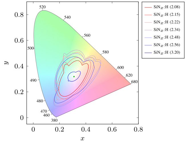
Fig. 20. CIE1931 color space chromaticity for different Si N x :H ARC layers with an AM 1.5G irradiance (optical index at \lambda = 600 nm in brackets) when taking the EVA and glass layers into account. The green point in the center of the gamut corresponds the simulation with no ARC.
