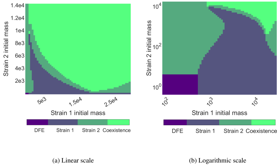
Fig. 8: Representation of the basins of attraction of the different equilibria in the two-strain case, in linear scale (8a) and logarithmic scale (8b). The parameters used are described in Table 1. Each strain is initialized with its steady state proportions (see Section 2.1) and diluted with a specific rate (between 1 and 1.10^{-5} ), and V is initialized to the disease-free value \lambda/\gamma . The axes represent the initial mass of each strain, i.e. the initial value of P + S for each strain (Strain 1 on the horizontal axis, Strain 2 on the vertical axis). The colors represent the outcome of the simulation (with colorbar above), one strain only or the two strains stably coexisting. Notice that the disease-free equilibrium is observed only in the bottom left corner
