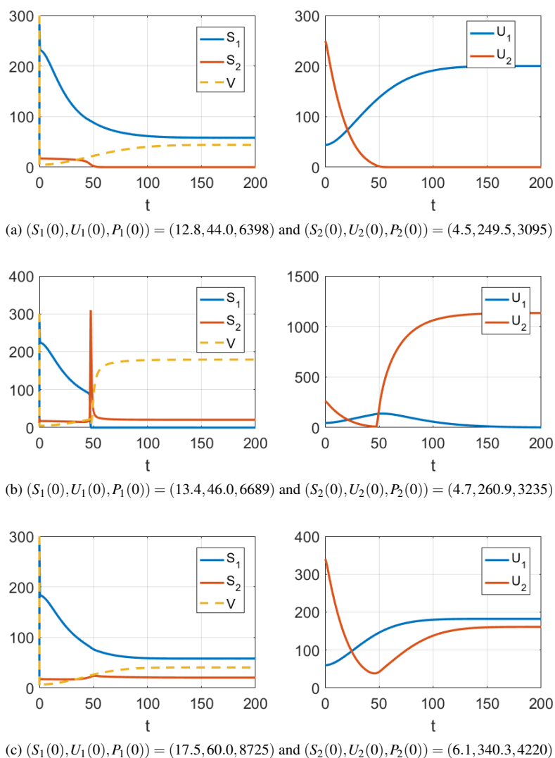
Fig. 9: Illustrations of typical cases from the diagram shown in Figure 8, representing the time evolution of the two strains (blue line is Strain 1, orange line is Strain 2). The parameters used are shown in Table 1. In each case, V is initialized to the disease-free steady-state \lambda/\gamma , and the strains are initialized with the specified conditions. The top panel (a) shows takeover of Strain 1, the middle panel (b) shows takeover of Strain 2, whereas the bottom panel (c) shows asymptotic coexistence of both strains.
