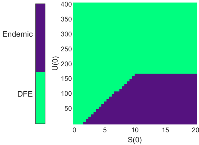
Fig. 7: Representation of the basins of attraction of the endemic steady-state (dark color) and the disease-free steady-state (lighter color), according to the initial condition. The horizontal axis represents the initial number of subunits, and the vertical axis represents the initial number of aggregates. The parameters used are those of Strain 1 in Table 1, the initial value for V is set to \lambda/\gamma (disease-free value), and the initial value for P is set to (2x_0 + \mu/\beta)U(0) (steady-state mean size)
