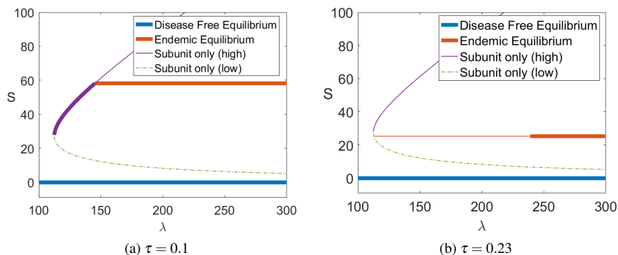
Fig. 3: Bifurcation diagram obtained for the steady-state subunit populations S when the monomer source, \lambda , varies for two values the polymerization rate \tau . The other parameters are set as in Table 1 (Strain 1). The four different equilibria are depicted (disease-free equilibrium, endemic equilibrium, higher subunit only equilibrium ( S_+ ), lower subunit only equilibrium ( S_- )). A thin line indicates an unstable equilibrium, whereas a bold line indicates a locally stable equilibrium
