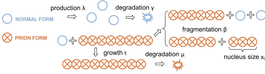
Fig. 1: Nucleated polymerization model with a single prion strain, illustrated with a nucleus size of x_0 = 3 . The normal form monomers (empty circles) appear with a production rate \lambda and are degraded with a rate \gamma . They are recruited by prion aggregates (crossed circles) with rate \tau . Each link in an aggregate may break with probability \beta , and an aggregate below the nucleus size x_0 is disassembled into normal monomers. The aggregates are degraded with rate \mu .
