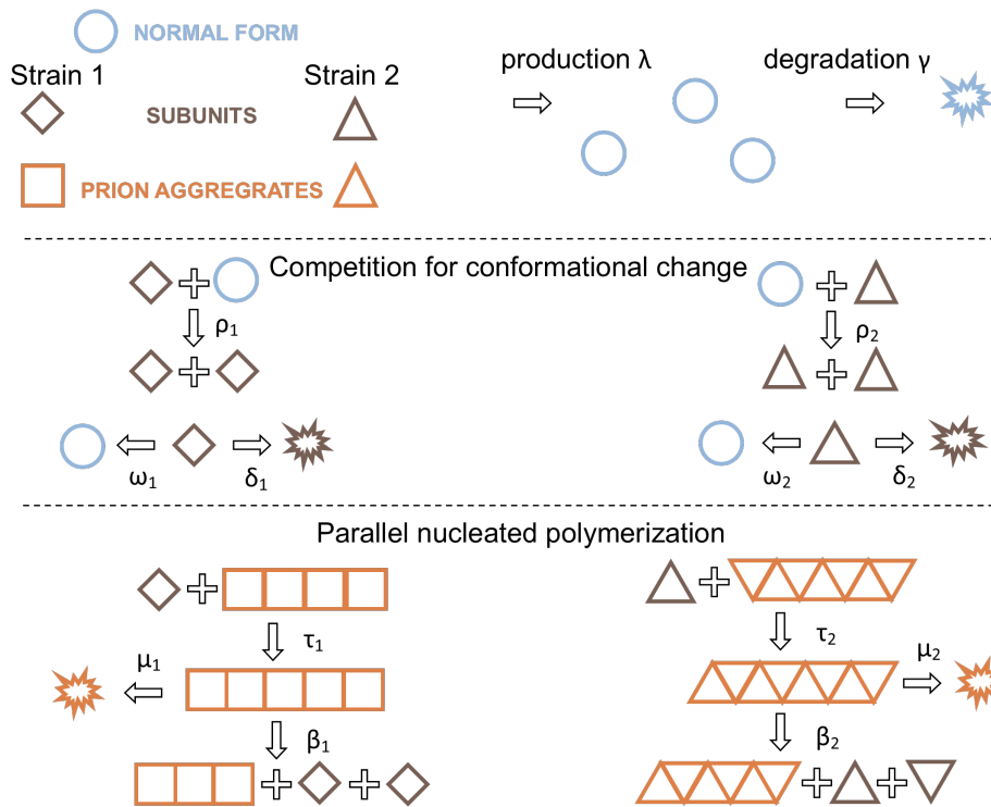
Fig. 5: Template assistance mechanism illustrated with two different strains (squares and triangles). The strains compete for normal monomers through the interaction with subunits (with rates \rho_1 and \rho_2 ). The dynamics of each strain taken individually are then described as in Figure 2.
