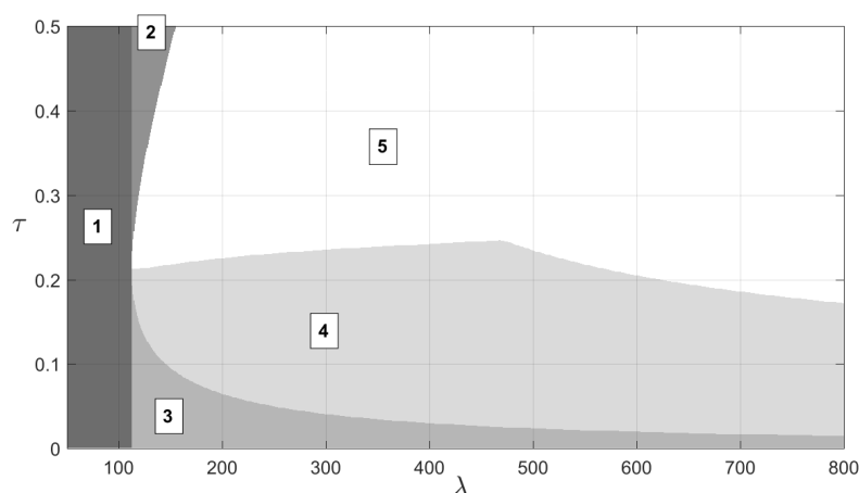
Fig. 4: Two-parameter bifurcation diagram obtained for the monomer source rate \lambda and the polymerization rate \tau , when the other parameters are described in Table 1 (Strain 1). The vertical line delimits the apparition of the subunit only equilibria, left of that line ( Region 1 ) only the disease-free equilibrium exists and it is then globally stable (not proved). The branches delimit the existence of the endemic equilibrium. In Region 2 , the subunit only equilibria exist but neither is stable. In Region 3 , the subunit only equilibria exist and the higher one ( S_+ ) is locally stable. In-between the branches, the endemic steady-state exists, but it is only locally stable in Region 4 . In Region 5 , the endemic steady-state is unstable. The boundary between Regions 4 and 5 corresponds to a Hopf bifurcation
