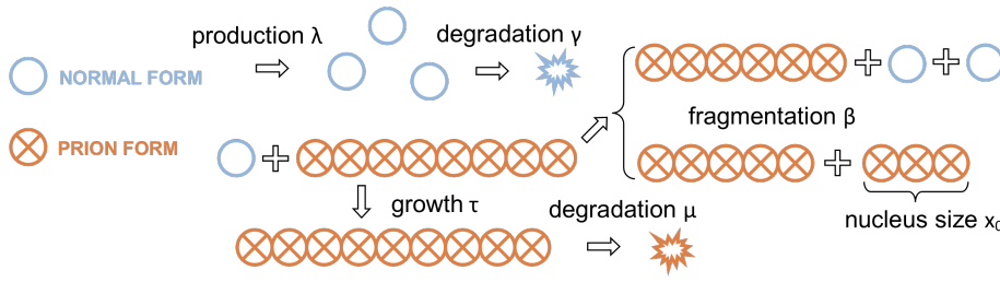
Fig. 1: Nucleated polymerization model with a single prion strain, illustrated with a nucleus size of x_0 = 3 . The normal form monomers (empty circles) appear with a production rate \lambda and are degraded with a rate \gamma . They are recruited by prion aggregates (crossed circles) with rate \tau . Each link in an aggregate may break with probability \beta , and an aggregate below the nucleus size x_0 is disassembled into normal monomers. The aggregates are degraded with rate \mu .
