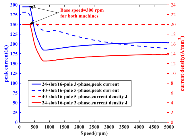
Fig. 17. Evolution of the peak current value and current density over the speed range for the three-phase and the five-phase machines with voltage constraints for J_{max}=20A/mm^2 .
