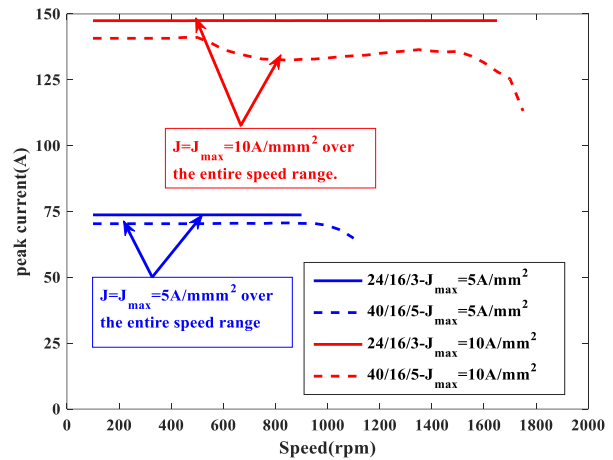
Fig. 16. Evolution of the peak current value and current density over the speed range for the three-phase and the five-phase machines with voltage constraints for J_{max}=5A/mm^2 and J_{max}=10A/mm^2 .
