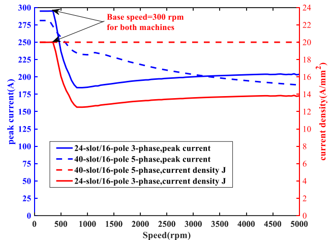
Fig. 17. Evolution of the peak current value and current density over the speed range for the three-phase and the five-phase machines with voltage constraints for J_{max}=20A/mm^2 .
