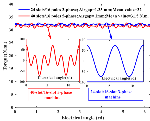
Fig. 14. Comparison of the delivered torque and the time domain current waveforms between the three-phase with 1.33 mm airgap and the five-phase machine with 1 mm airgap with J=5A/mm^2 .
