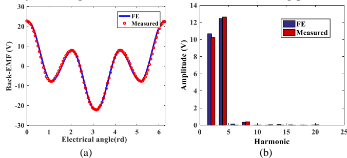
Fig. 7. (a) back-EMF at no-load (b) harmonics.
