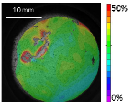
Fig. 1 : Inflation test on the hepatic capsule, first principal strain field E1 before failure
