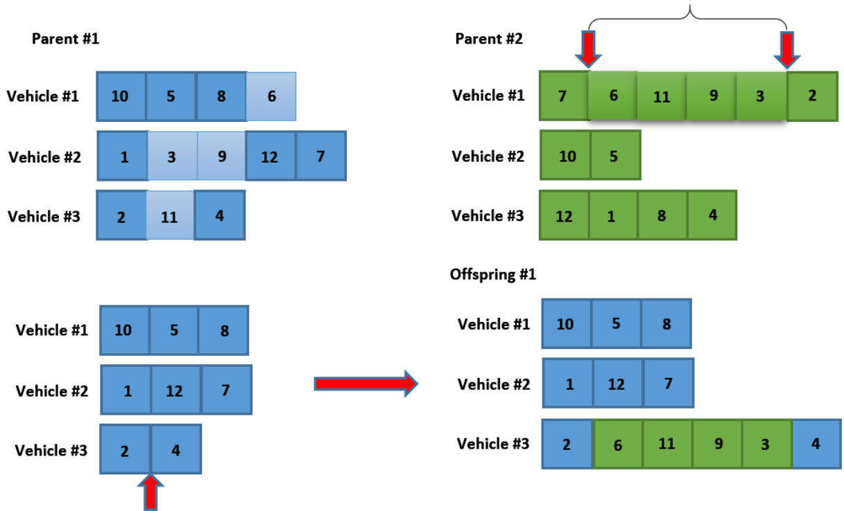
Figure 5. Random Crossover operator
