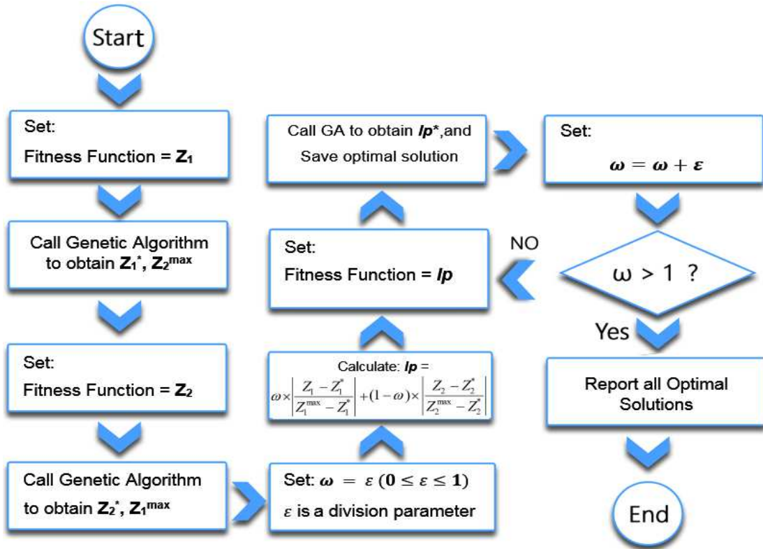
Figure 3. The flowchart of hybrid GA
