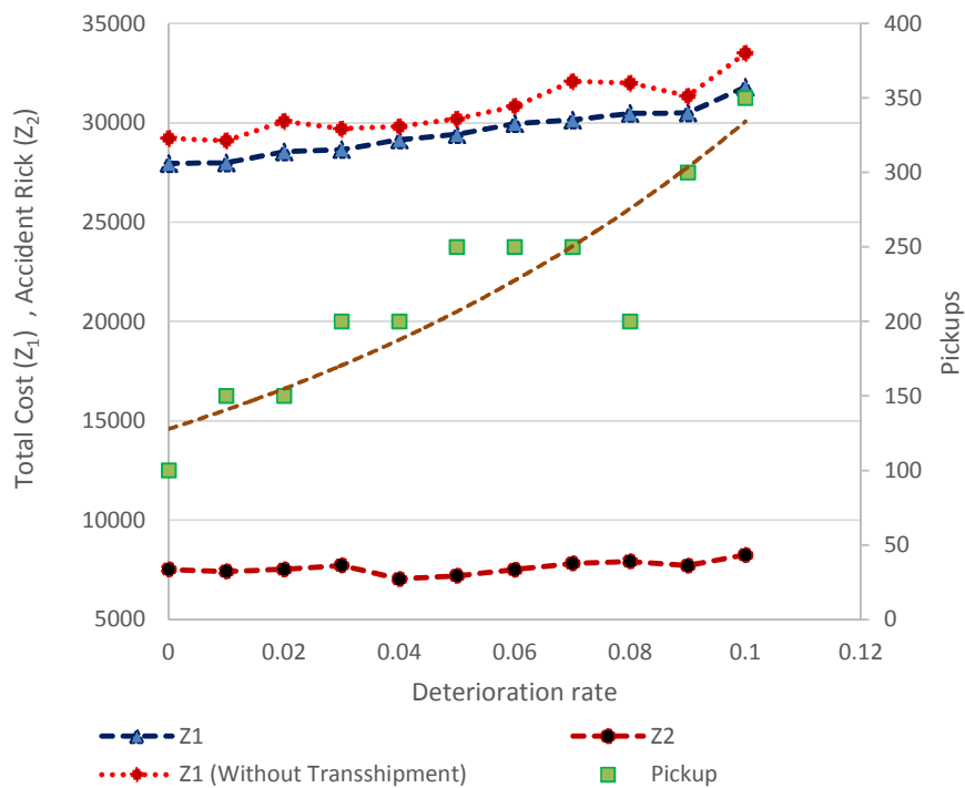
Figure 6. Accident loss and total cost as a function of the deterioration rate
