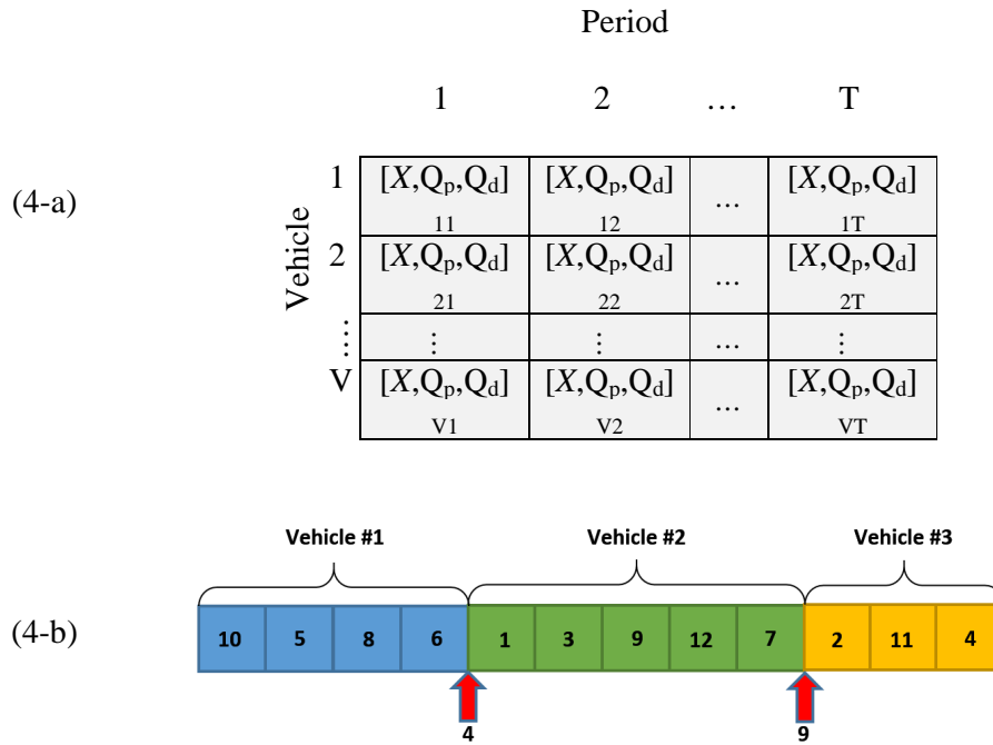
Figure 4. The solution and chromosome structure
