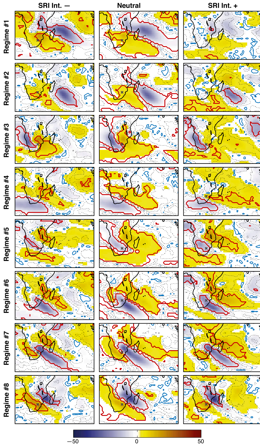
FIG. 10. Daily OLR anomalies ( W m^{-2} ) during the occurrences of the eight convective regimes during the (left) negative, (central) neutral, and (right) positive phases of the SRI index filtered at the interannual time scale (shown in Fig. 1a) according to the multimember ensemble mean of 20CR. Only anomalies that are significant at the 95% significance level according to a t test are displayed. The blue cross shows the Gauteng province of South Africa discussed in the text.
