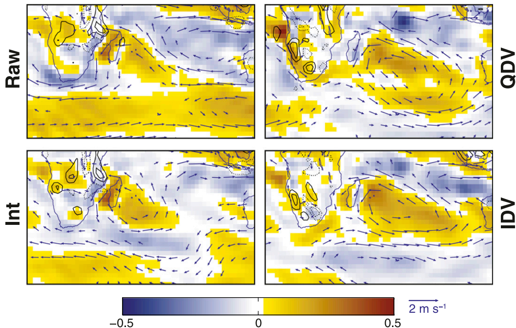
FIG. 11. As in Fig. 9, but for 850-hPa horizontal wind anomalies, during the positive phase of the raw and filtered SRI indices. Contours show associated divergence (convergence) anomalies ( s^{-1} ): solid (dotted) contours denote divergence (convergence) anomalies. Contour interval is every 5 \times 10^{-2} s^{-1} , and the zero contour is omitted. Shadings show associated vorticity anomalies ( s^{-1} ). All analyses are based on 20CR ensemble mean. Only anomalies that are significant at the 95% significance level according to a t test are displayed.
