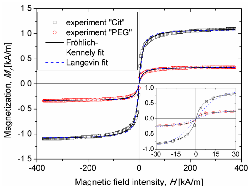
Figure 2. Magnetization curves of aqueous suspensions of multicore IONPs covered by either citrate anions or PEG. Inset shows a zoomed view of magnetization curves at low magnetic fields. Symbols correspond to experimental data, solid line—Fröhlich–Kennely fit, and dashed line—Langevin fit.
