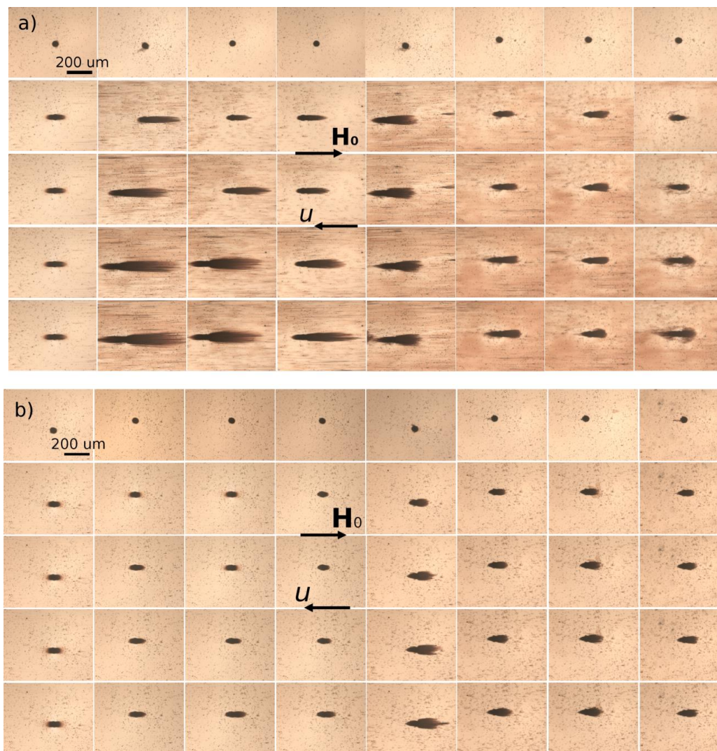
Figure 6. Snapshots of the deposits of citrated (a) or PEGylated (b) IONPs around a single magnetized micropillar in the microfluidic channel under hydrodynamic flow and externally applied magnetic field of intensity H_0 = 13.5 kA/m at the nanoparticle volume fraction \varphi_0 = 0.17 \pm 0.03 vol.%. The rows of (a) and (b) correspond to different elapsed times: from the top to the bottom t = 0, 10, 20, 40, and 60 min; the columns correspond to different flow speeds u = 0, 0.714, 1.43, 2.14, 2.85, 5.23, 7.61, and 10 mm/s.
