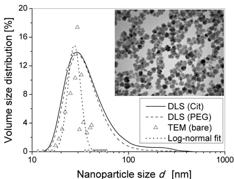
Figure 1. Volume size distribution of multicore iron oxide nanoparticles (IONPs) measured by DLS and TEM. The hydrodynamic size distribution was measured by DLS on IONPs coated by either citrate anions (Cit sample—continuous line) or PEG (PEG sample—dashed line). The TEM size distribution (triangles) was obtained on bare IONPs by analysis of the TEM micrograph shown on the figure inset, followed by conversion of the number size distribution to the volume size distribution for comparison with distributions of the coated IONPs by DLS using Mie theory. The TEM volume size distribution was fitted by log-normal law (dotted line, Equation (1)).
