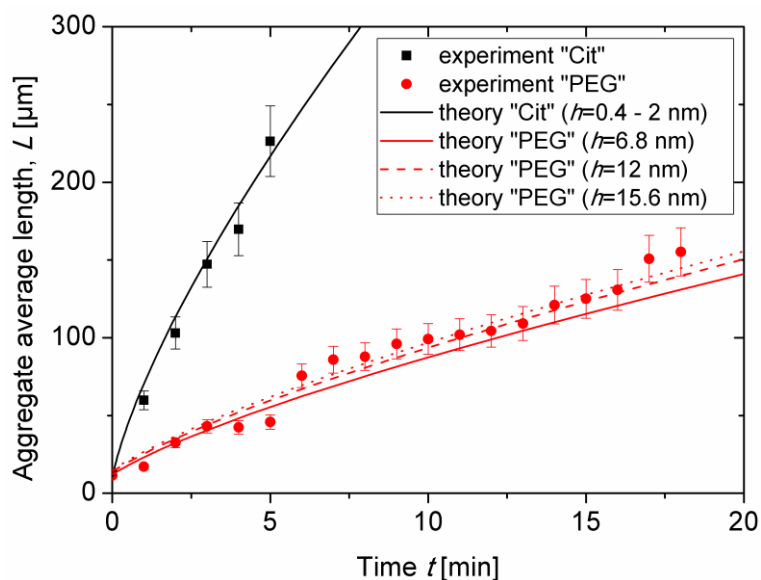
Figure 5. Experimental and theoretical dependencies of the aggregate length on the elapsed time since the beginning of magnetic field application for the citrated and the PEGylated samples respectively, at the same nanoparticle volume fraction \varphi_0 = 0.17 \pm 0.03 vol.% and at the intensity of the applied magnetic field H_0 = 13.5 kA/m.
