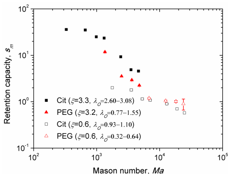
Figure 9. Mason number dependencies of the retention capacity of citrated and PEGylated nanoparticles at different values of the parameters \zeta and \lambda_O .
