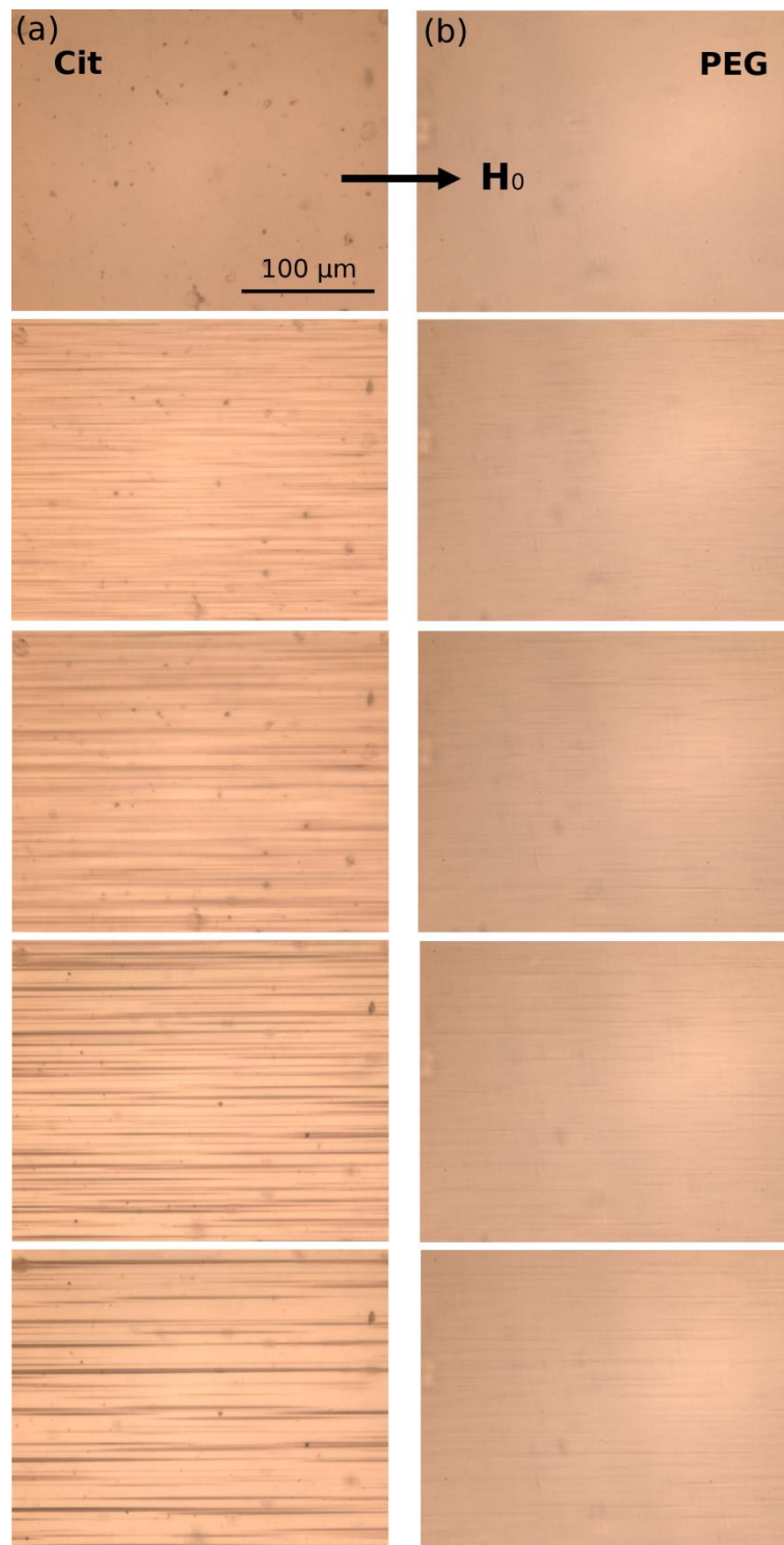
Figure 4. Snapshots of aqueous suspensions of citrated (a) and PEGylated (b) IONPs at particle volume fraction \varphi_0 = 0.17 \pm 0.03 vol.% subjected to an external uniform magnetic field of intensity H_0 = 13.5 kA/m. Each row corresponds to the elapsed time from the moment of the magnetic field application t = 0 (upper row), 5, 10, 15 and 20 min (bottom row).
