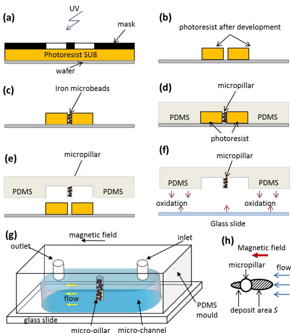
Figure 3. Principle stages of microfabrication of a microfluidic channel for magnetic separation (a–f). The sketch of the microfluidic channel is presented in (g). The deposits of IONPs around the micropillar is presented schematically in (h); the deposit surface area S is hatched.
