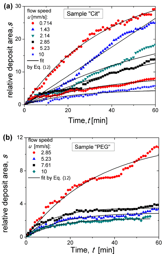
Figure 7. Time dependences of the relative deposit area for the Cit (a) and the PEG (b) samples at the applied magnetic field intensity H_0 = 13.5 kA/m and for different flow speeds. Symbols correspond to experiments, solid lines correspond to the fit by Equation (12).
