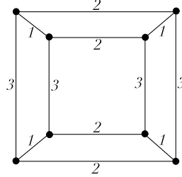
FIGURE 1. This labelled graph will be employed in more than one construction in the present paper.
