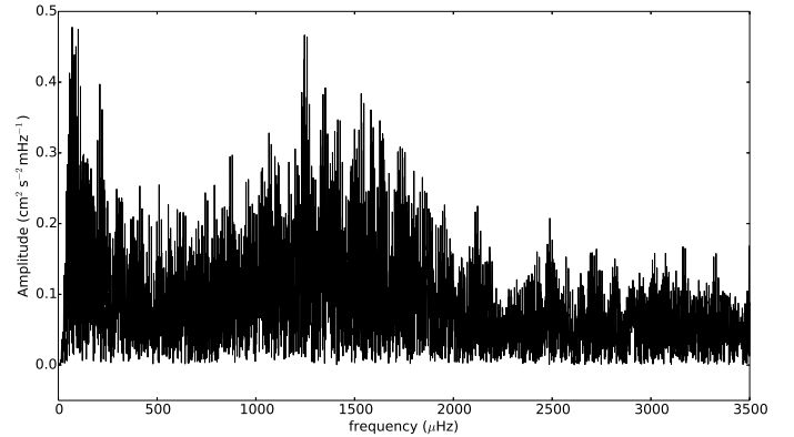
Fig. 1. Global Fourier transform of 94 Ceti data.
