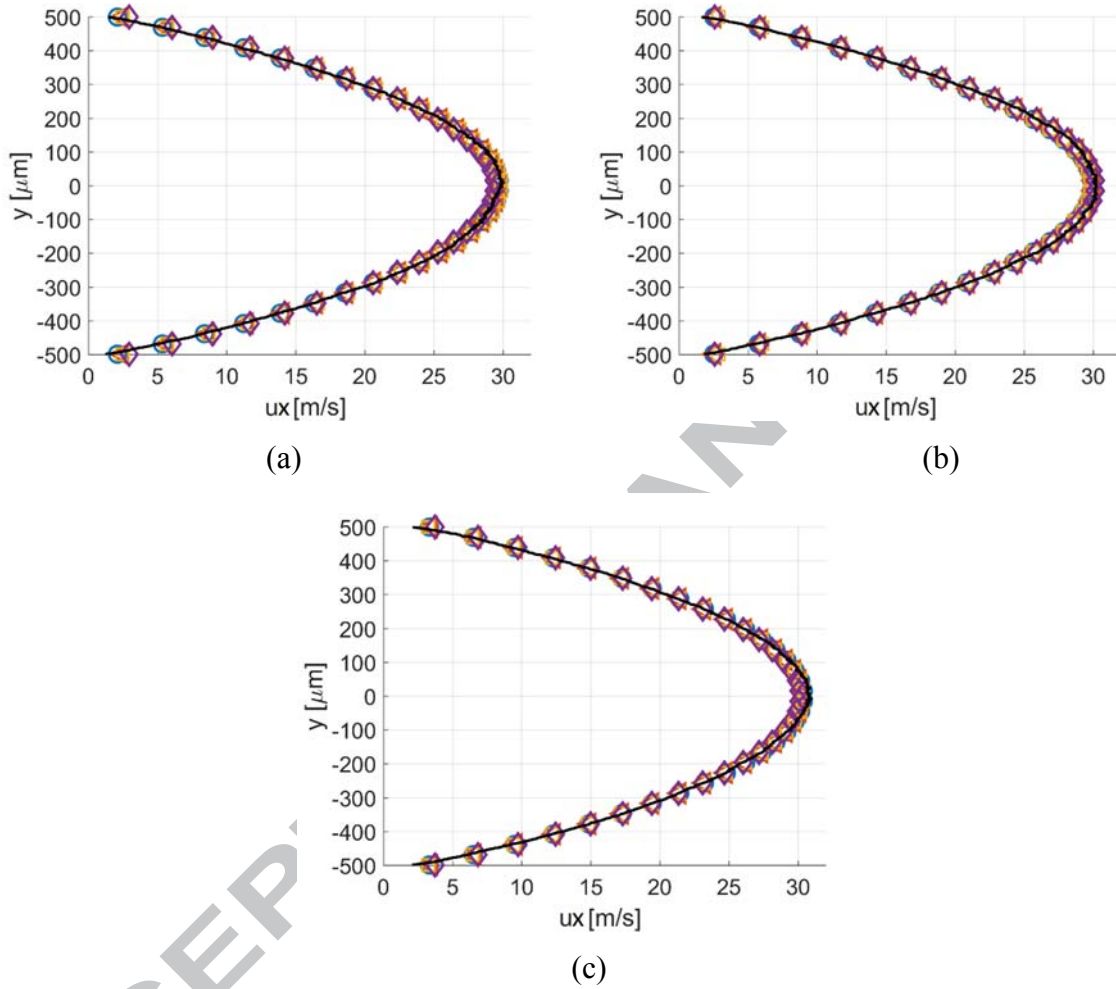
Figure 17. Comparison between DSMC (black solid line) and reconstructed velocity profiles for times t = 10 \mu\text{s} ( \circ ), 25 \mu\text{s} ( \triangleleft ), 50 \mu\text{s} ( \square ), 100 \mu\text{s} ( \diamond ) and for (a) Kn = 0.015 , (b) Kn = 0.02 , and (c) Kn = 0.025 .
