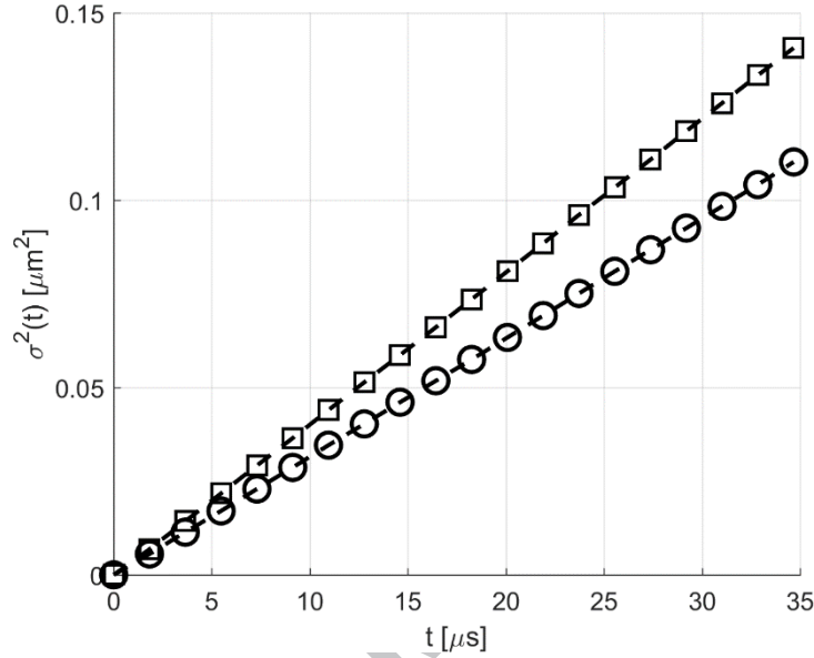
Figure 15. Evolution in time of the variance \sigma(t)^2 of the tracer molecules position, as defined in Eq. (13), for (O) acetone-helium and (□) diacetyl-helium mixtures with a tracer concentration \chi = 5\% and Kn = 0.02 .
