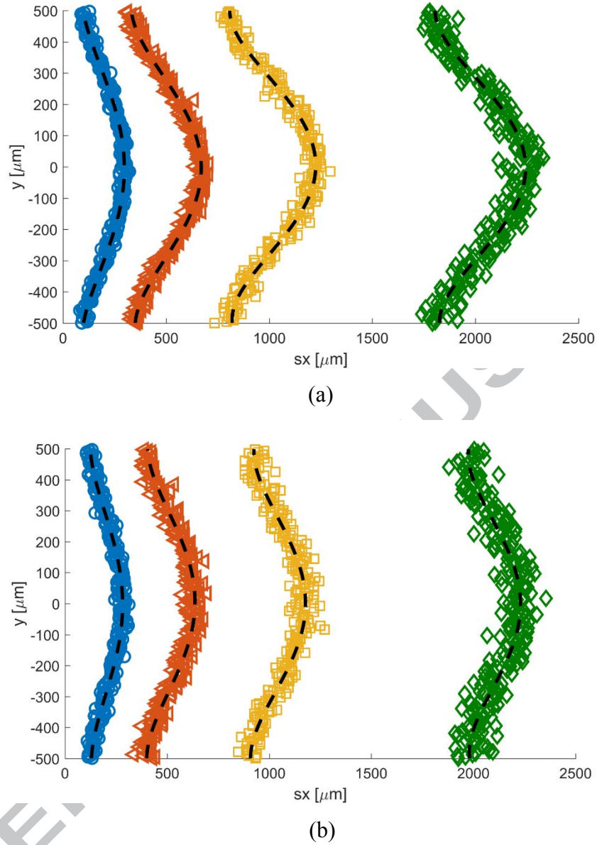
Figure 13. Displacement data s_{xj} from DSMC simulation (symbols) of acetone-helium mixture with \chi_2 = 5\% for (a) Kn = 0.015 and (b) Kn = 0.025 , at times t = 10 \mu\text{s} ( \circ ), 25 \mu\text{s} ( \triangleleft ), 50 \mu\text{s} ( \square ), 100 \mu\text{s} ( \diamond ) after the acetone molecules tagging. The black dashed line is the displacement profile s_x(y) given by the data polynomial fitting.
