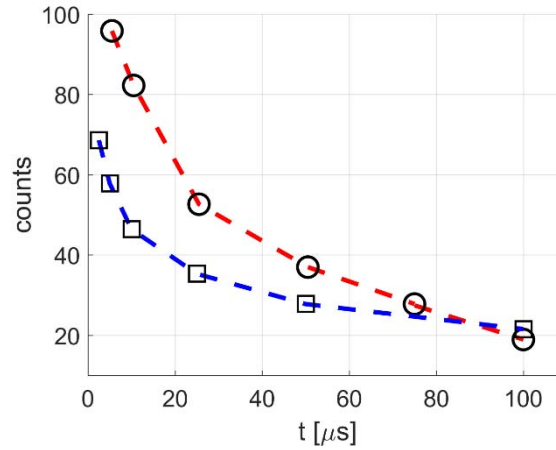
Figure 10. Time evolution of phosphorescence emission in helium for acetone (O - -) and diacetyl ( \square - -) at p = 1 kPa and T = 293 K. For the data on acetone emission:
