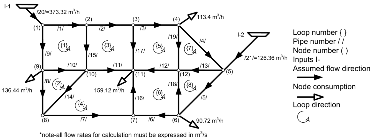
Fig. 3. Example of looped gas distributive pipeline network
