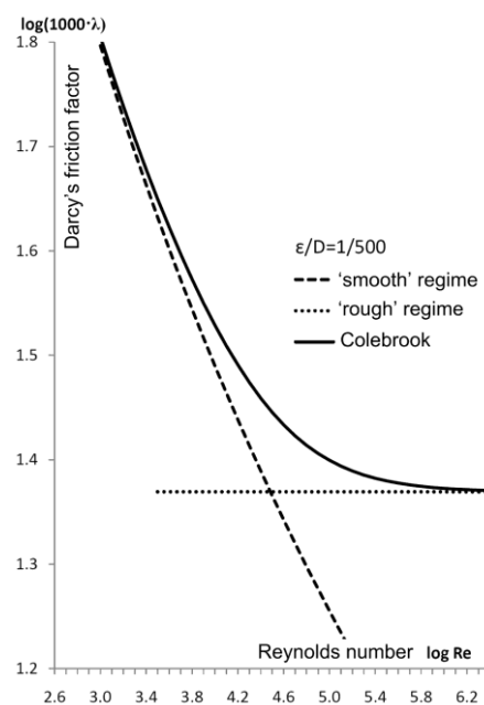
Fig. 1. Colebrook relation make transitional curve among hydraulically "smooth" regime and turbulent rough regime
