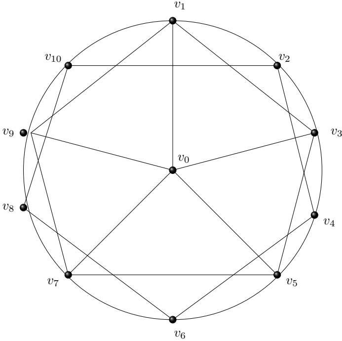
Figure 3: Anti-web gear graph ( AWG_5 )
