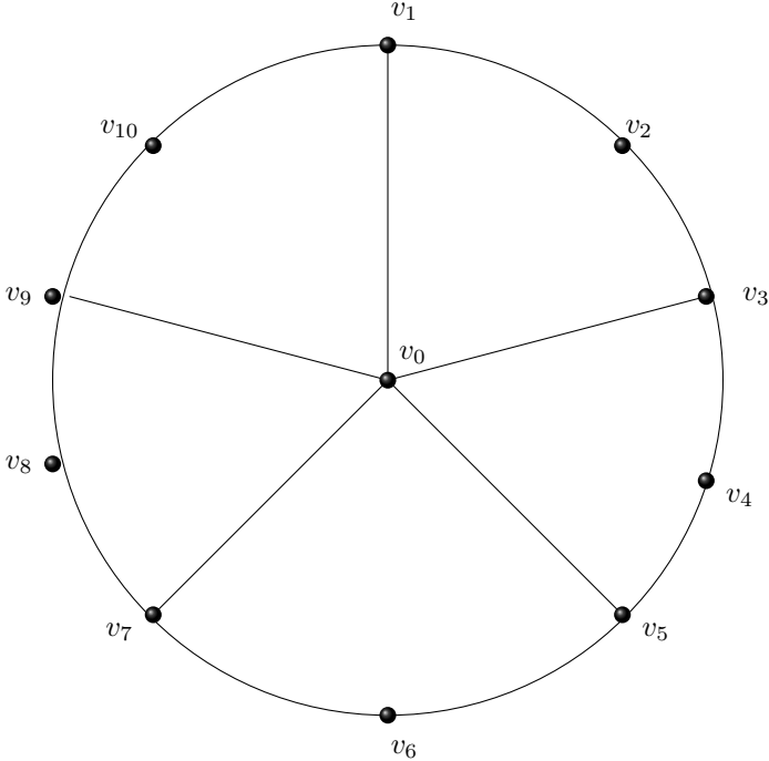
Figure 1: Gear graph ( G_5 )
