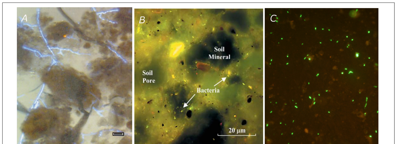
FIGURE 8 | Examples of experimentally determined microbial distribution in soils: (A) microscopic image of hyphae of the fungus Rhizoctonia solani growing in the pore space of a sandy loam. Scale bar 20 \mu\text{m} (Harris et al., 2002. Reproduced with permission of the British Mycological Society). (B) Micrograph of ethidium bromide-stained thin sections of a silt loam soil after inoculation by Escherichia coli . Image obtained using an epifluorescence microscope with blue excitation (Modified from Li et al., 2004. Reprinted with permission). (C) CARD-FISH stained Bacillus subtilis cells in soil filter sections under double excitation filter 643 (465–505 and 564–892 nm) (Modified from Juyal et al., 2018).
