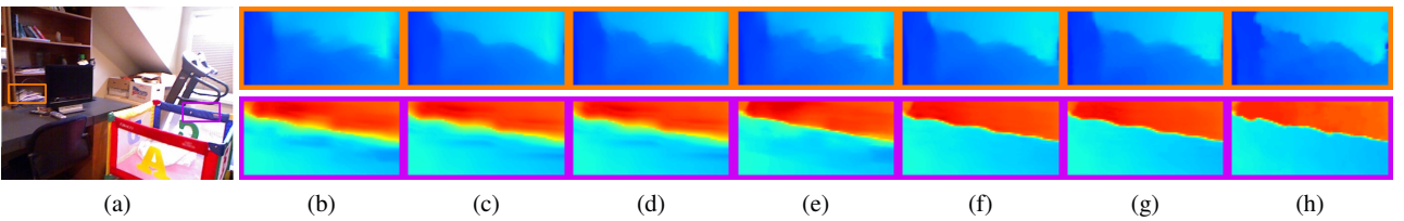
Fig. 13 Visual comparison of different networks (DKN) for depth upsampling ( 8\times ) using the kernel of size 3 \times 3 . (a) a RGB image. Results for weight regression using (b) RGB, (c) depth and (d) RGB and depth images. Results for weight and offset regression using (e) RGB, (f) RGB and depth images, and (g) RGB and depth images with the residual connection. (h) ground truth.
