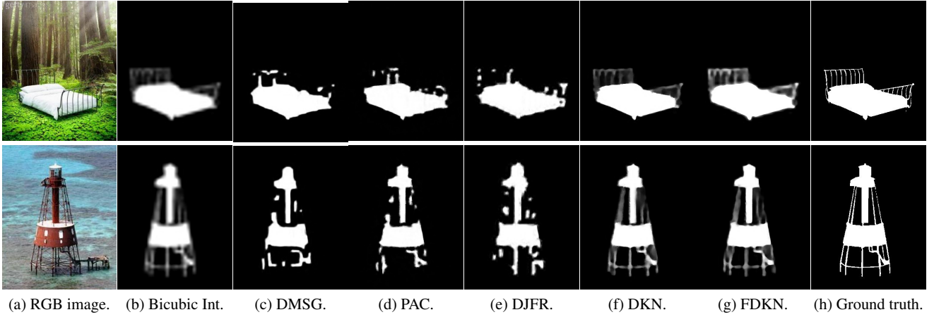
Fig. 9 Visual comparison of saliency map upsampling ( 8\times ) on the DUT-OMRON dataset (Yang et al. 2013): (a) a RGB image, (b) Bicubic Int., (c) DMSG (Hui et al. 2016), (d) PAC (Su et al. 2019), (e) DJFR (Li et al. 2019), (f) DKN, (g) FDKN, and (h) ground truth.
