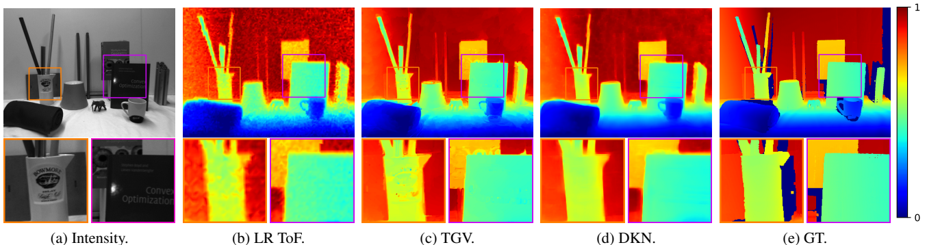
Fig. 9 Visual comparison of noisy depth map upsampling on the books sequence in the ToFMark dataset (Ferstl et al. 2013): (a) Intensity, (b) LR ToF, (c) TGV (Ferstl et al. 2013), (d) DKN, and (e) GT.
