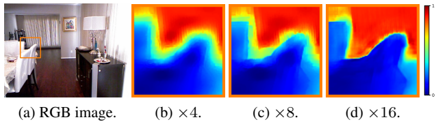
Fig. 16 Visual comparison of upsampled depth images for DKN when the scale factors for training ( \times 16 ) and test ( \times 4, \times 8, \times 16 ) are different.
