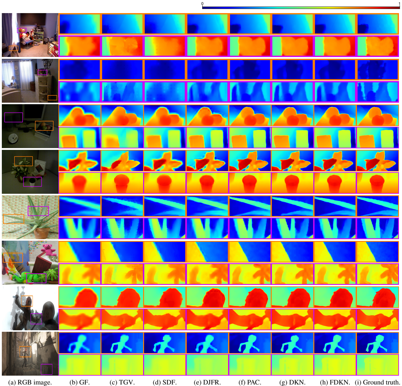
Fig. 6 Visual comparison of upsampled depth images ( 8\times ): (a) an RGB image, (b) GF (He et al. 2013), (c) TGV (Ferstl et al. 2013), (d) SDF (Ham et al. 2018), (e) DJFR (Li et al. 2019), (f) PAC (Su et al. 2019), (g) DKN, (h) FDKN, and (i) ground truth. Top to bottom: Each two rows show upsampled images on the NYU v2 (Silberman et al. 2012), Lu (Lu et al. 2014), Middlebury (Hirschmuller and Scharstein 2007) and Sintel (Butler et al. 2012) datasets, respectively. Note that we train our models with the NYU v2 dataset, and do not fine-tune them to other datasets.
