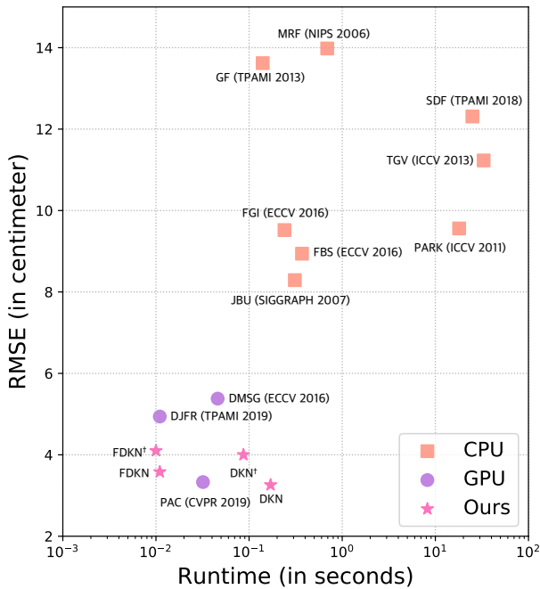
Fig. 15 Runtime and root mean squared errors (RMSE) comparison of upsampled depth maps ( 8\times ) on the NYU v2 (Silberman et al. 2012) dataset. †: Our models trained with the depth map only without any guidance.
