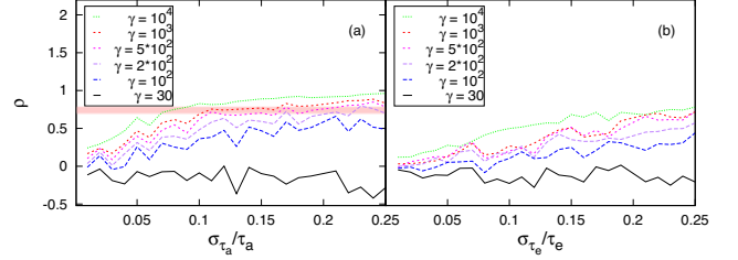
Figure 3. Spearman's rank correlation coefficient \rho of the flux-rms scatter plot as a function of (a) \sigma_{\tau_a}/\tau_a and (b) \sigma_{\tau_e}/\tau_e . The legends are same as in Fig. 1. The pink band shows the 1\text{-}\sigma ( 0.6325/\sqrt{N-1} ) error range for the observed value for Mkn421 (Section 3).
