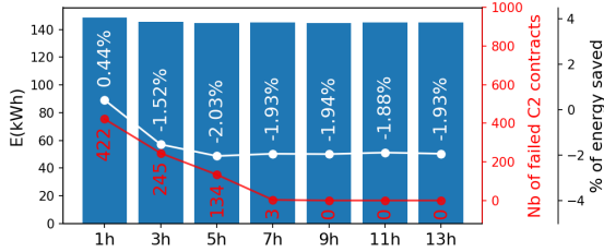
Figure 6: Percentage of energy saving with C2 contracts according to the allowed time window.
