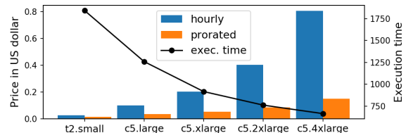
Figure 4: Execution time, hourly price and prorated price of Montage in all possible VM sizes.
