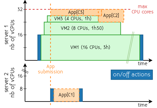
Figure 2: Possible scheduling ( execution contracts ) of an 8 vCPUs application in an infrastructure with 2 servers and 3 VMs. Starting the application at submission time (C1) requires to turn on server 2. Delaying (C2) or changing the size (C3) can avoid the need of server 2, thus saving energy.
