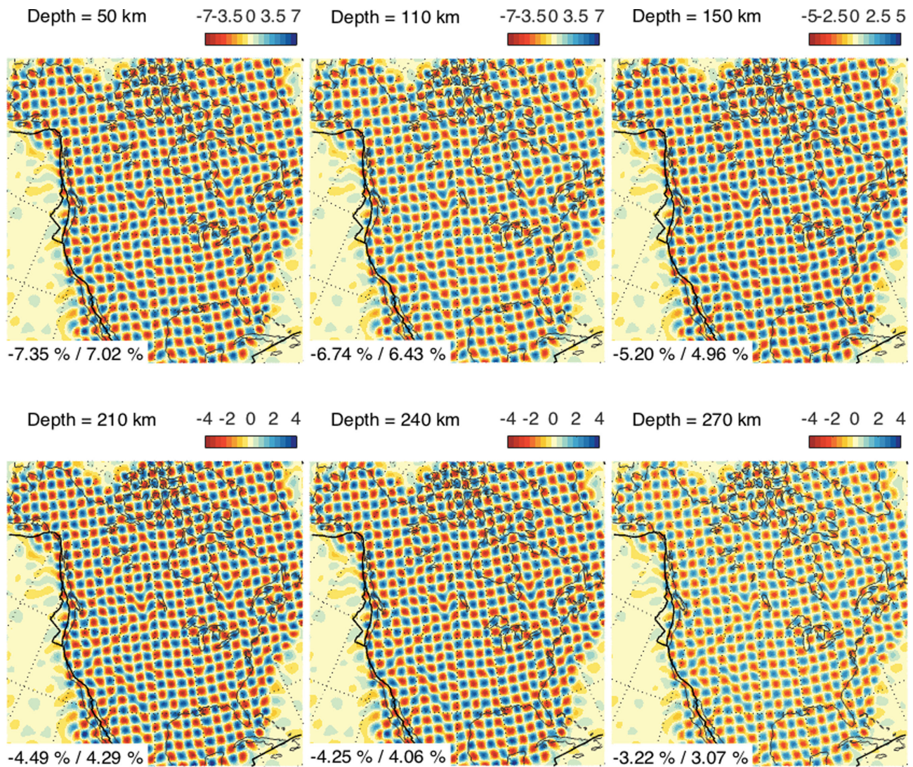
Figure A1. Input model for checkerboard tests of V_S in North America. Each checkerboard test model is constructed by assigning a non-zero coefficient to a single radial spline v_q(r) (eq. 6), resulting in 3-D structure concentrated around the corresponding depth (shown at the top left). The lateral structure is obtained by assigning the same value but opposite signs to each spherical spline \beta_p(\theta, \varphi) (eq. 6) with 2^\circ node spacing. For each model, the structure is shown only at the depth corresponding to the maximum velocity perturbation. The colour bars, at the top right of each panel, indicates perturbations in per cent. Note that the scale is different in different panels. Minimum and maximum perturbations are indicated at the bottom of each map. Amplitudes of cells mimic amplitudes observed in the model presented in this study.
