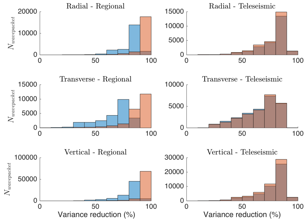
Figure 3. Histograms showing variance reduction between data and synthetics by component, separating the teleseismic and regional data sets. The y-axis gives the number of wavepackets and the x-axis is the variance reduction in per cent. The variance reduction is defined (as in Table 1 as 100 \times (1 - wr^2) ) where wr are the weighted residuals. The left-hand column shows variance reductions for regional events and the right-hand column for teleseismic (outside of RegSEM chunk) events. In each panel, blue/red bins show waveform variance reductions for the starting model and the current model, respectively. Dark red allows to see blue bins behind red bins. Variance reduction is much less significant for the teleseismic data, as the misfit is mostly due to the model outside of the region of study, which has been kept fixed.
