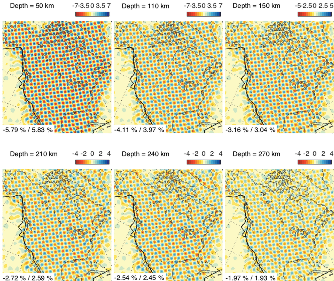
Figure A2. Output model for checkerboard tests of V_S in North America, corresponding to the input models shown in Fig A1. Presentation is as in Fig. A1. We calculate the resolving power of the inversion by using classical linear resolution analysis (e.g. Tarantola 2005), whereby we construct the resolution matrix corresponding to the last iteration of our inversion. While structures show good spatial recovery, amplitudes – due to application of damping during the inversion – is generally reduced. The recovery is poorer in the northern part of the continent (between Greenland and North America especially) as expected from our density and azimuthal coverage (see Fig. 4). In the future, the use of out-of-box stations in our Box Tomography inversion procedure will greatly improve the illumination of this area while keeping its cost low.
