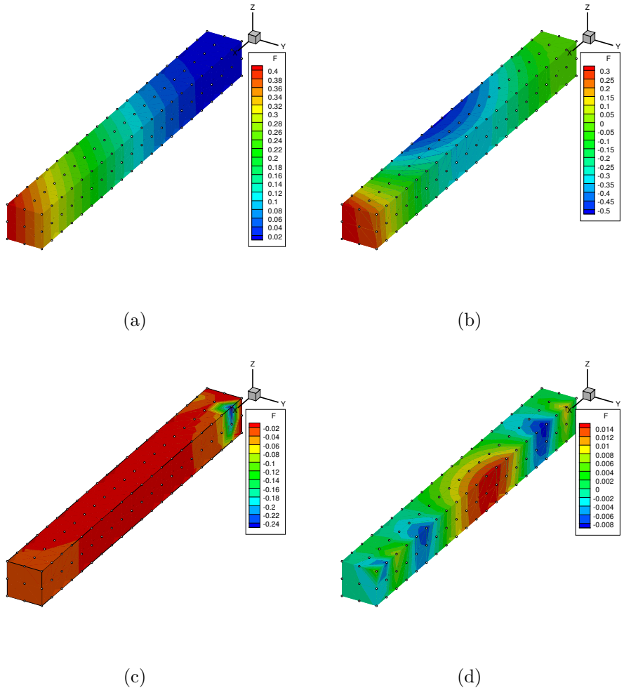
Figure 2: First two modes of the beam model, depending on the physical coordinates \boldsymbol{x} (top) and load position \boldsymbol{s} (bottom).
