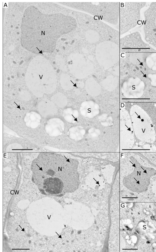
Figure 2. Representative transmission electron microscopy images of the root statocytes of Brassica napus seedlings with the presence of potassium pyroantimonate (PA) precipitates. Images are shown for seedlings grown in simulated gravity (A–C), microgravity (D) or after simulated gravity removal ( 1g_s + \mu g , E–G). Thanks to the electron-dense structure, PA precipitates are visible as spherical black dots and were mainly observed in the cytosol (A and E). Some precipitates were detected near statoliths, inside the vacuoles (D) and the nucleus (F). No precipitates were found either in the cell wall (B) or in the statoliths (C). Arrows indicate examples of PA precipitates in various cellular components. C: cytosol; CW: cell wall; N: nucleus; S: statoliths; V: vacuole. Bar scales indicate 2\mu m .
