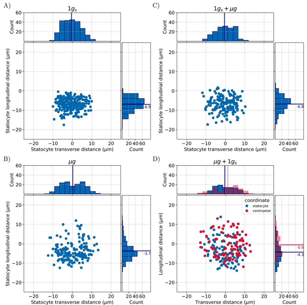
Figure 3. Stalolith positioning within root statocytes. The position of each stalolith is indicated in blue and is given relative to the statocyte centroid (0,0) along the cell transverse and longitudinal directions. Data are shown for each condition: 1g_s (A), \mu g (B), 1g_s + \mu g (C), \mu g + 1g_s (D) and are accompanied by a histogram of counts along each direction. In the \mu g + 1g_s (D) condition, red spots indicate the position of staloliths along the centrifugation force (centripetal coordinates). Solid lines and values indicate the means of counts for each condition.
