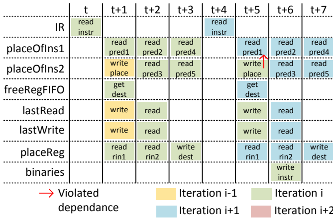
Fig. 8. Schedule of the different memory operations of IRScheduler with initiation interval at 4.
