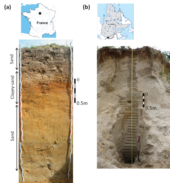
Fig. 1. Locations and photographs of the trenches where sand samples were taken for soil water extraction and water isotope analysis for (a) the Paris Basin and (b) the St. Lawrence Lowlands.
