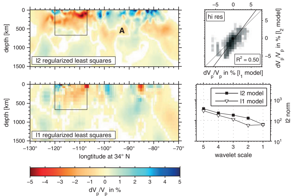
Figure 6. Cross section through the velocity models at 34^\circ\text{N} (see Figure 1 for location). The top left panel is the cross section in the Sigloch [2008] model. The bottom left one is from this study. In the top right, we represent the values of the velocities as a density scatterplot for the well-resolved (hi-res) part, a total least-squares regression line through the data (thick black line) and the one-to-one line for reference (thin black line). The well-resolved part (rectangles) is located below the dense network in the upper mantle. The remainder of the model domain is less well resolved. In the bottom right, we show energy spectra of the heterogeneity in both cross sections, as the \ell_2 norms of their wavelet coefficients for different scales. See text for details.
