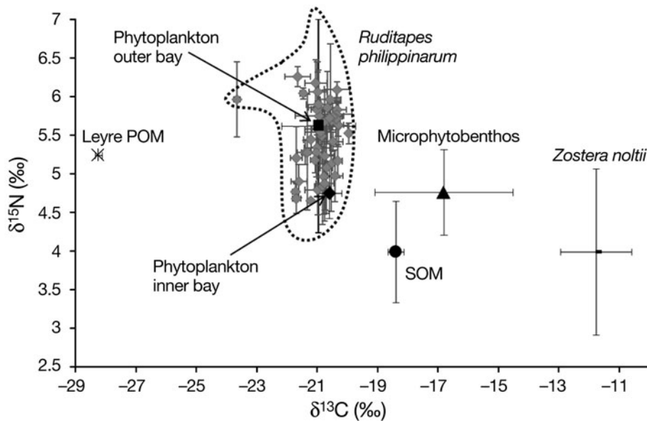
Fig. 5. Ruditapes philippinarum . N vs. C stable isotope ratios (mean \pm SD) of posterior adductor muscles of clams sampled at 50 stations (corrected for trophic shift; \diamond ) and trophic sources potentially consumed as inner bay phytoplankton-dominated particulate organic matter (POM; \blacklozenge ), outer bay phytoplankton-dominated POM ( \blacksquare ), Leyre POM ( \times ), microphytobenthos ( \blacktriangle ), sediment ( \bullet ) and Zostera noltii ( - ). The area enclosed by the dotted line corresponds to the expected \delta^{13}\text{C} and \delta^{15}\text{N} of the food resources incorporated by the Manila clam in its adductor muscle, as deducted from trophic shifts of 3.5 and 3‰ for \delta^{13}\text{C} and \delta^{15}\text{N} , respectively
