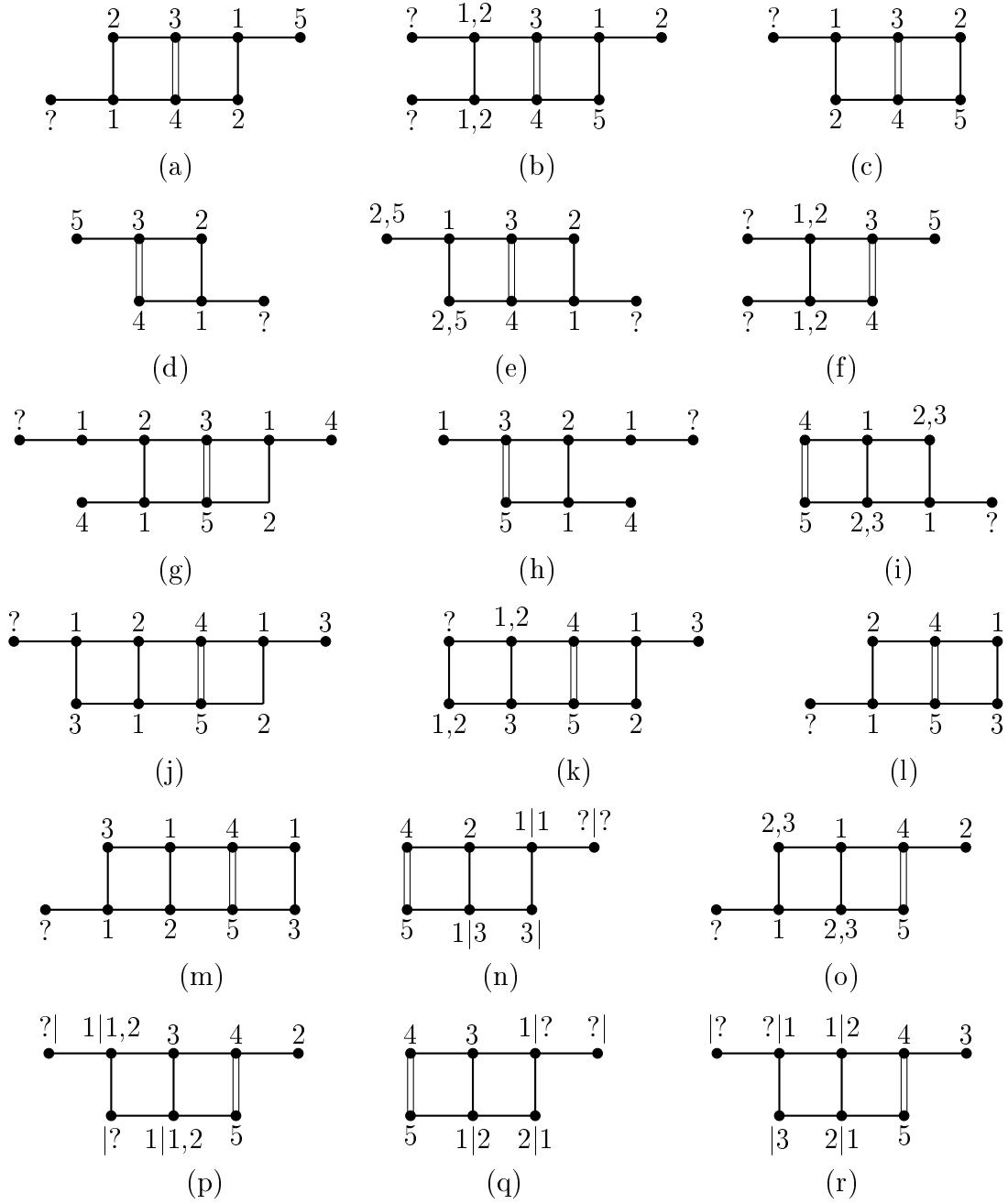
Figure 19: Configurations for the proof of Lemma 4 (the double edge is the edge u_i v_i ).
