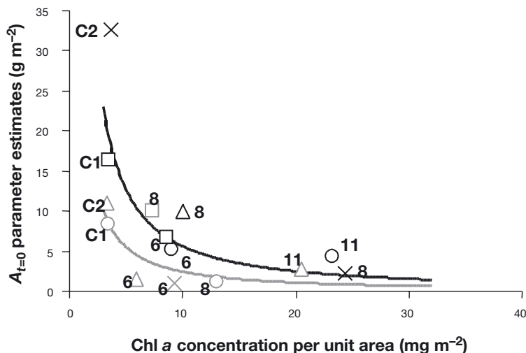
Fig. 4. Estimates of the A_{t=0} parameter (i.e. the amount of sediment in the fluff layer) with and without snails (black and grey symbols, respectively). Lines represent the minimized relationship (Eq. 11) between these estimates and sediment surface (section 0–2 mm) chl a concentrations per unit area ( mg\ m^{-2} ) with and without Hydrobia ulvae bioturbation (black and grey lines, respectively). Symbols correspond to the same experiments as in Fig. 1
