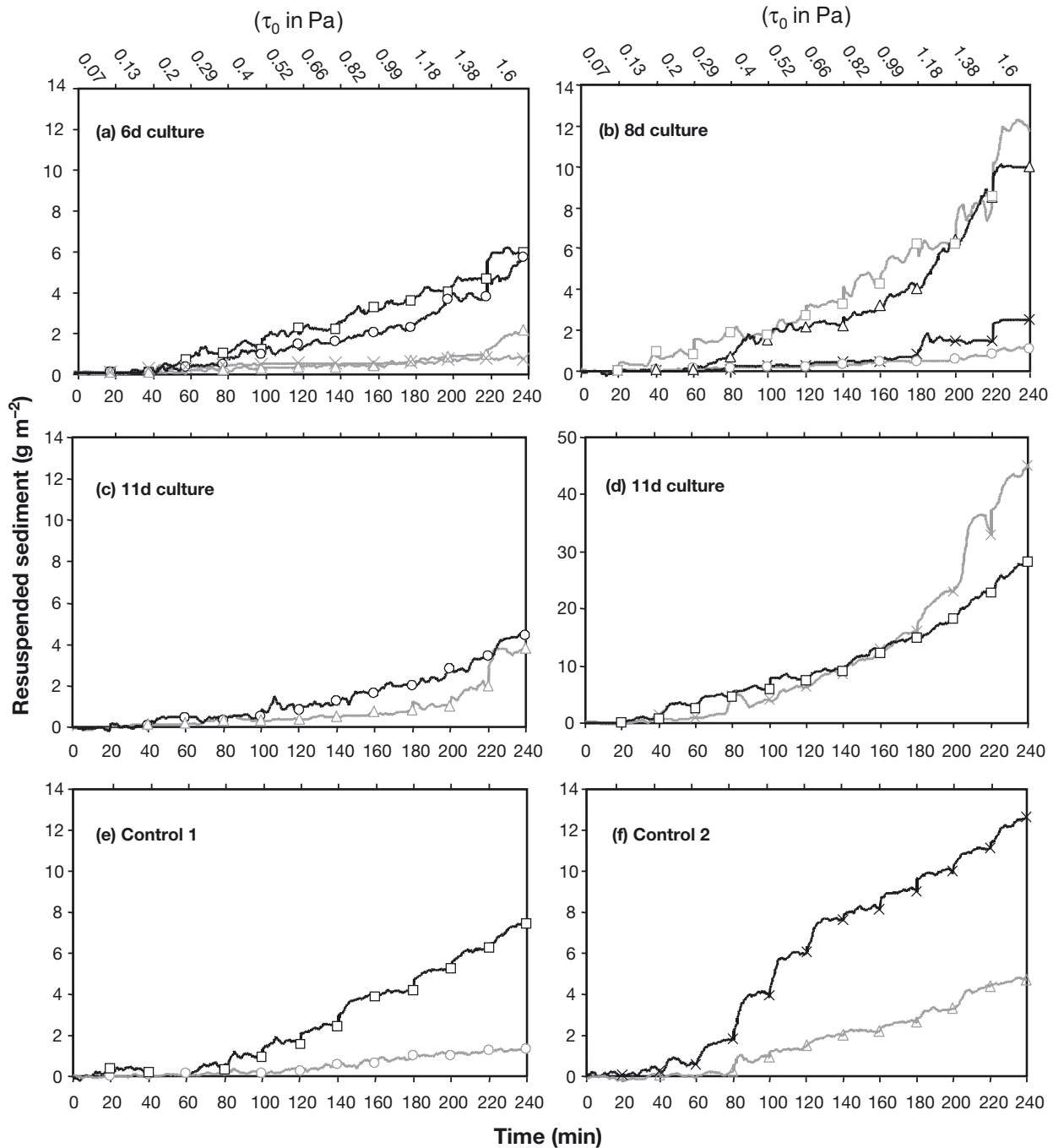
Fig. 3. Sediment resuspension with and without Hydrobia ulvae bioturbation (in black and grey, respectively) after (a) 6, (b) 8 and (c) 11 d of diatom growth and for (e) Control 1 and (f) Control 2 without diatoms. The 11 d culture experiments were separated into 2 pools: (c) those displaying fluff layer erosion and (d) those displaying Type I bed erosion (note the greater y-axis scale). Symbols correspond to the same experiments as in Fig. 1
