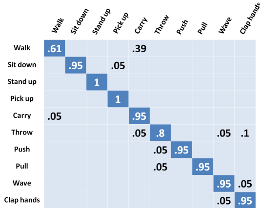
Fig. 4: Confusion matrix obtained on UTKinect dataset
