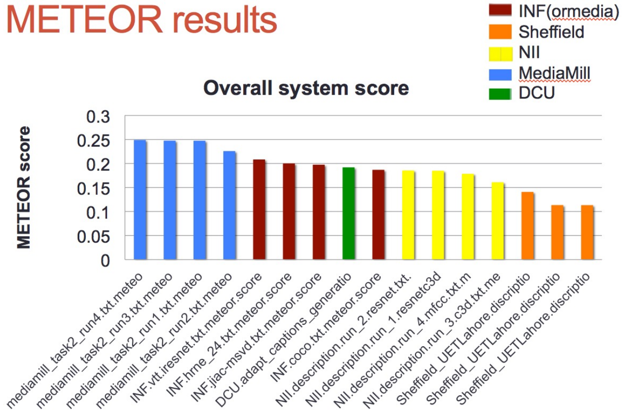
Figure 47: VTT: Results using the METEOR metric
