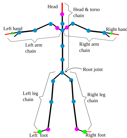
Fig. 3. Articulated chains and DOF controlled through IK. Red segments indicate end-effector associated to each articulated chain. Degrees of freedom of each joint are indicated as follows: green dots = 1 DOF, pink dots = 2 DOF, and light-blue dots = 3 DOF.
