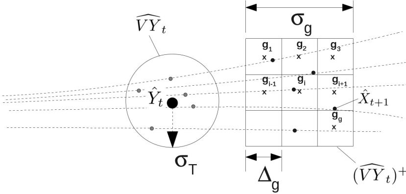
Fig. 4. Local grid bootstrap procedure
